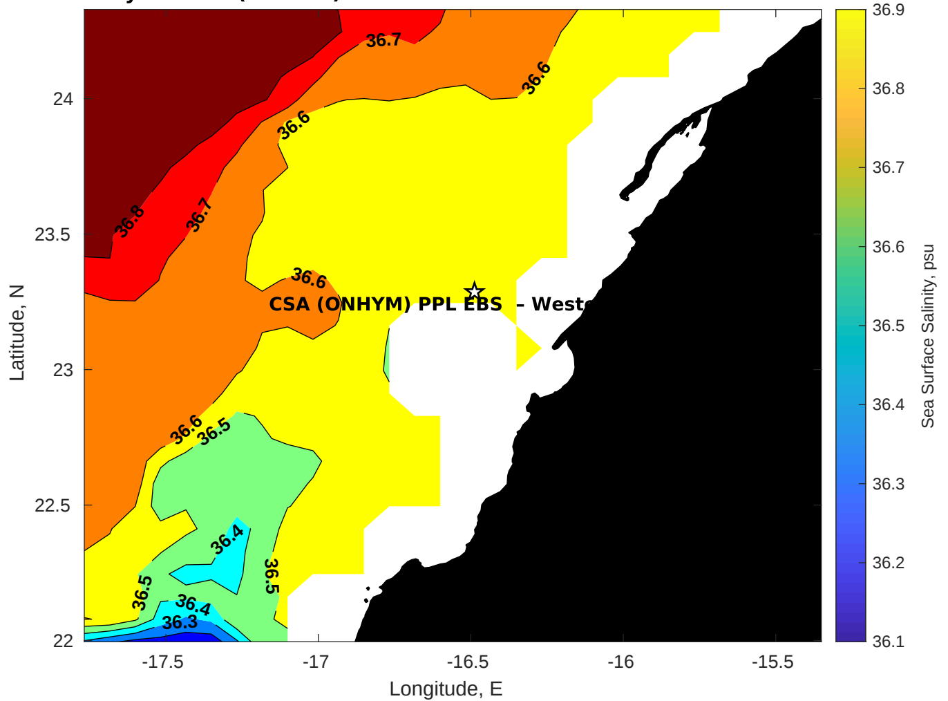
Surface Salinity for CSA (ONHYM) PPL EBS - Western Sahara at 28-Nov-2025 00:00:00
