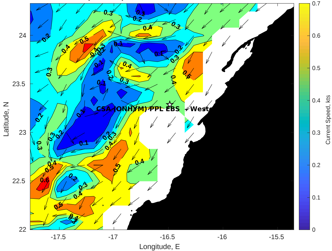
Surface Currents for CSA (ONHYM) PPL EBS - Western Sahara at 28-Nov-2025 00:00:00
