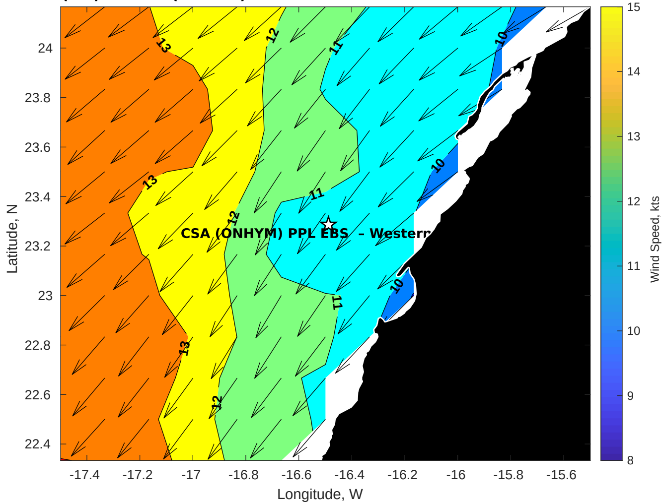
GFS Winds (kts) for CSA (ONHYM) PPL EBS - Western Sahara at 29-Nov-2025 09:00:00
