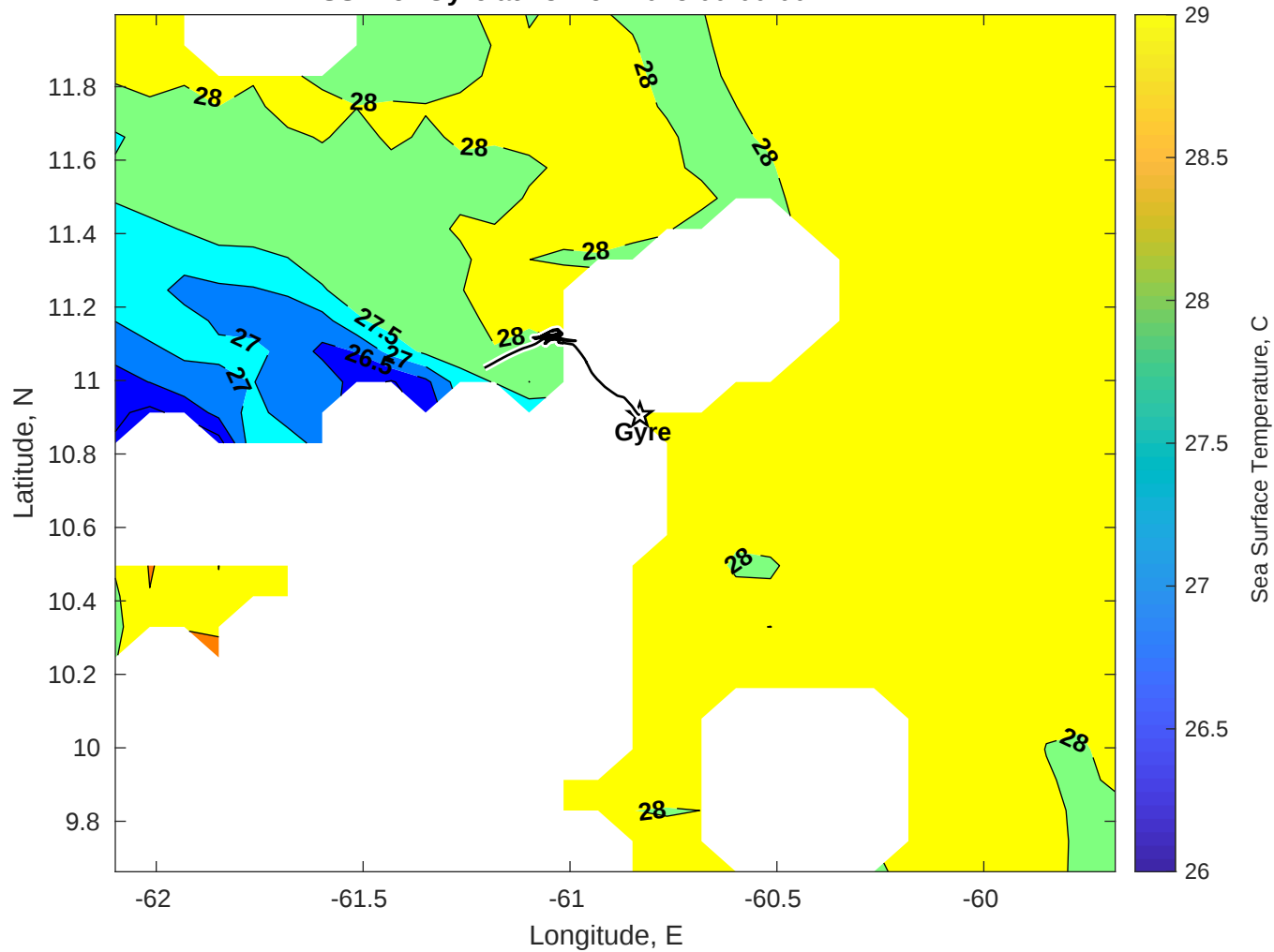
SST for Gyre at 28-Nov-2025 00:00:00
