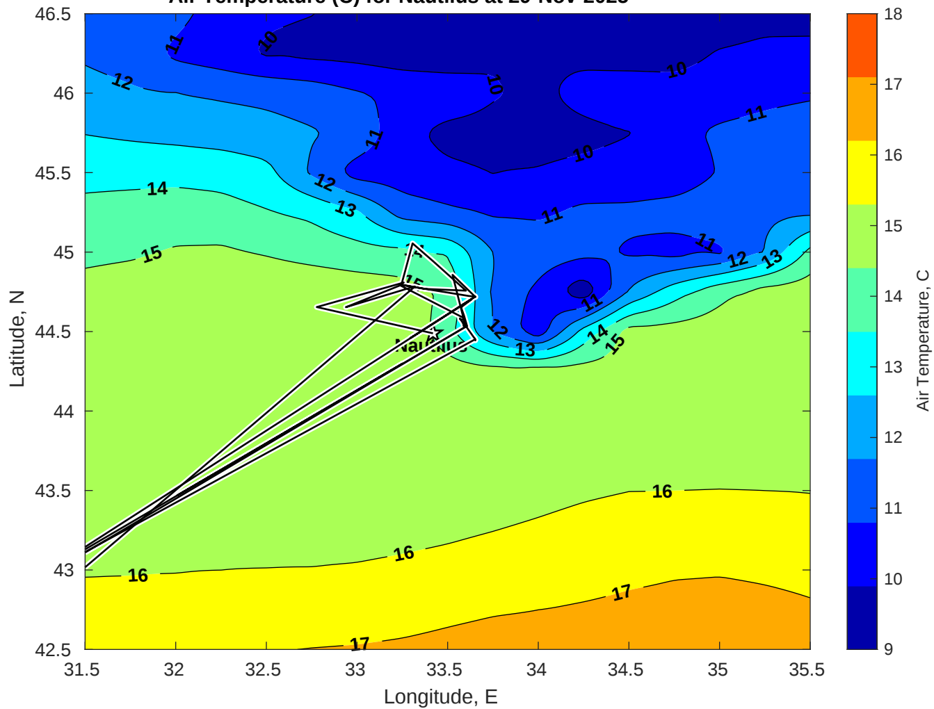
Air Temperature (C) for Nautilus at 29-Nov-2025
