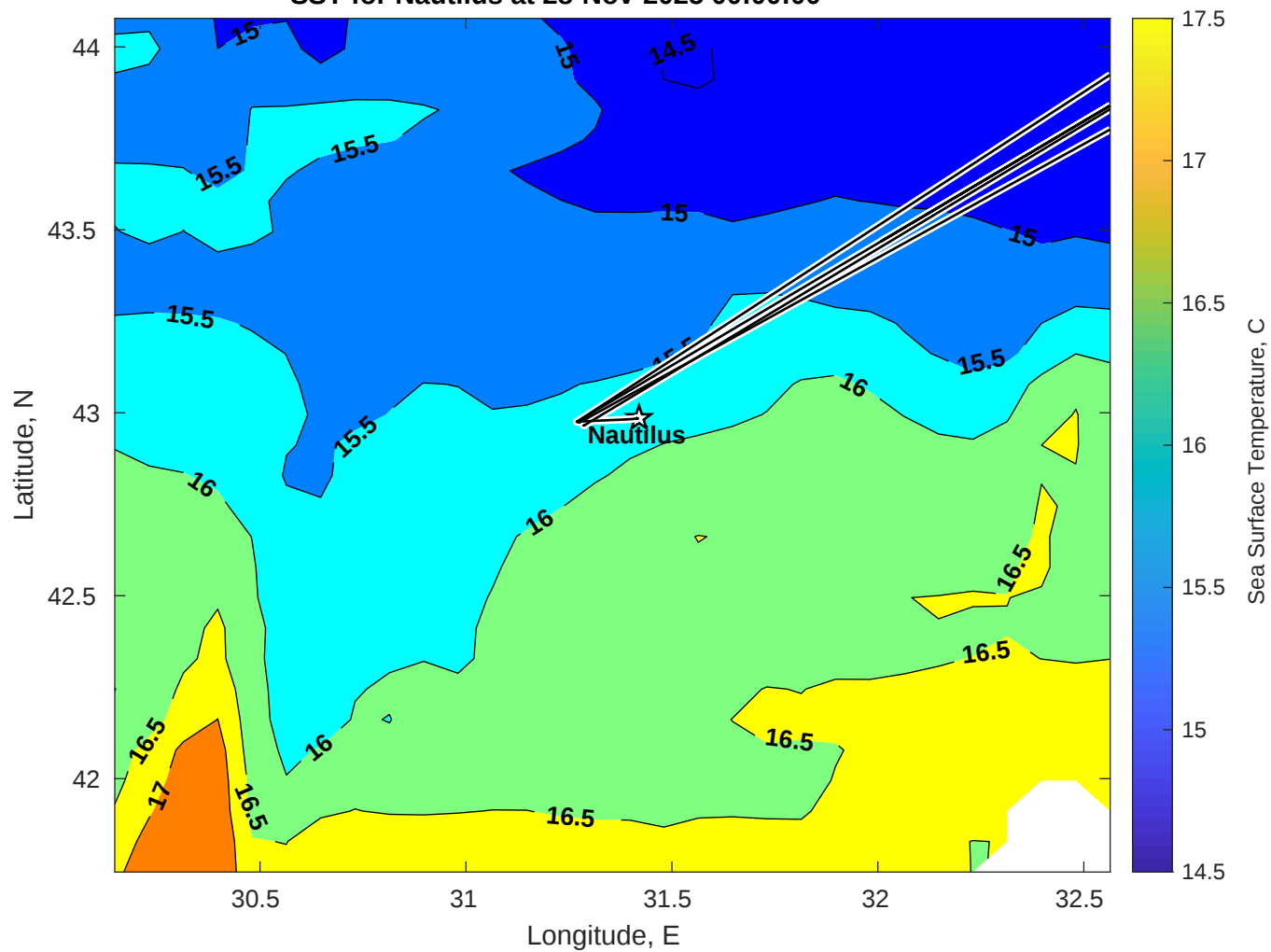
SST for Nautilus at 28-Nov-2025 00:00:00
