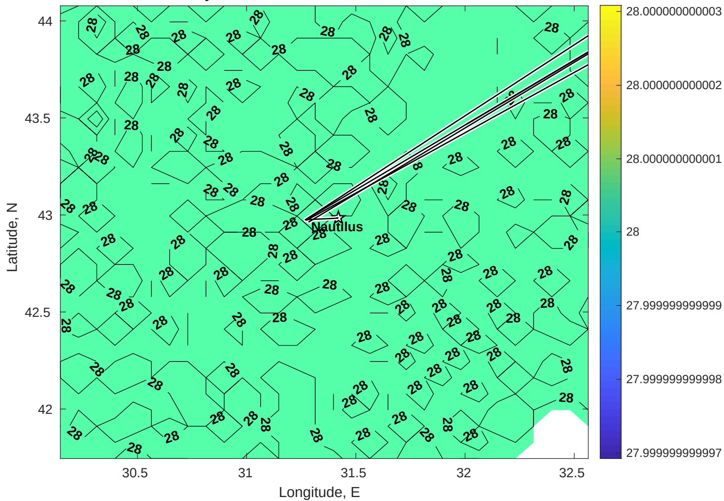
Surface Salinity for Nautilus at 28-Nov-2025 00:00:00
