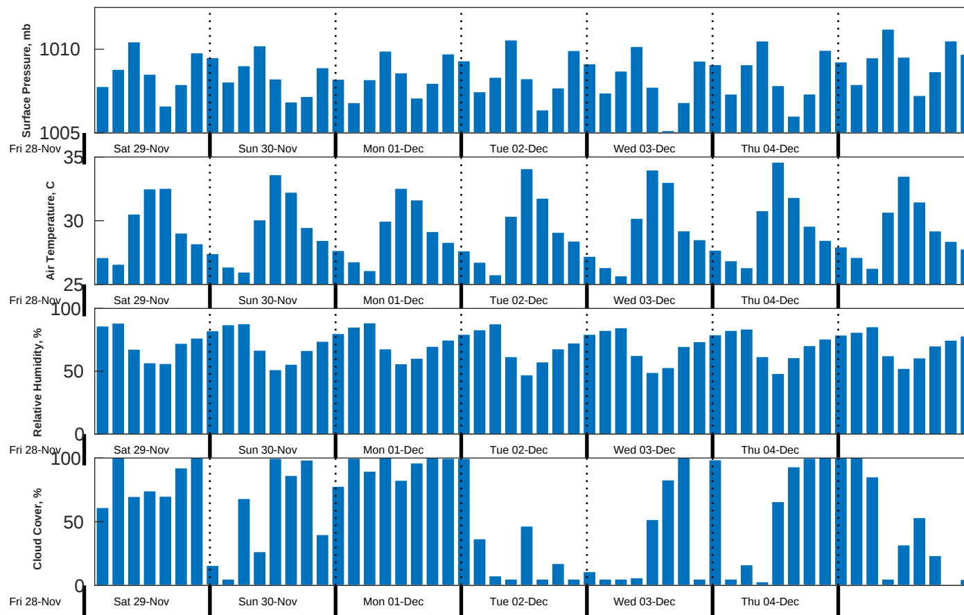
Met Forecast for Proteus from 29-Nov-2025 00:00:00 to 06-Dec-2025 00:00:00
