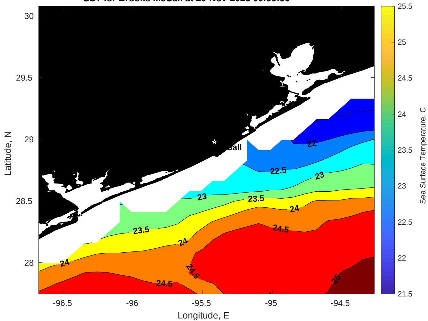
SST for Brooks McCall at 29-Nov-2025 00:00:00
