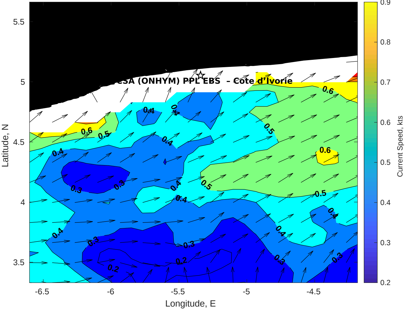
Surface Currents for CSA (ONHYM) PPL EBS - Cote d'Ivoire at 29-Nov-2025 00:00:00
