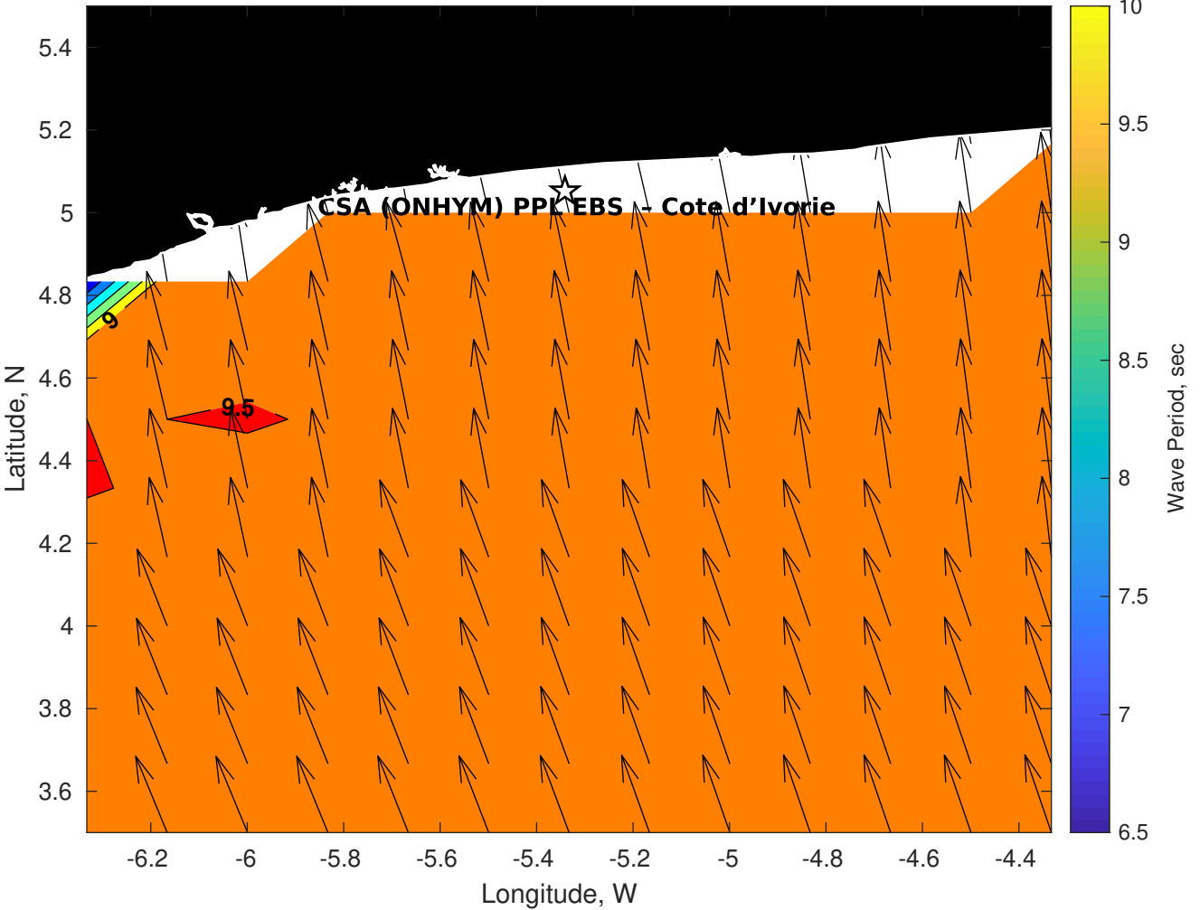
GFS Wave Period (sec) for CSA (ONHYM) PPL EBS - Cote d'Ivoire at 30-Nov-2025 09:00:00
