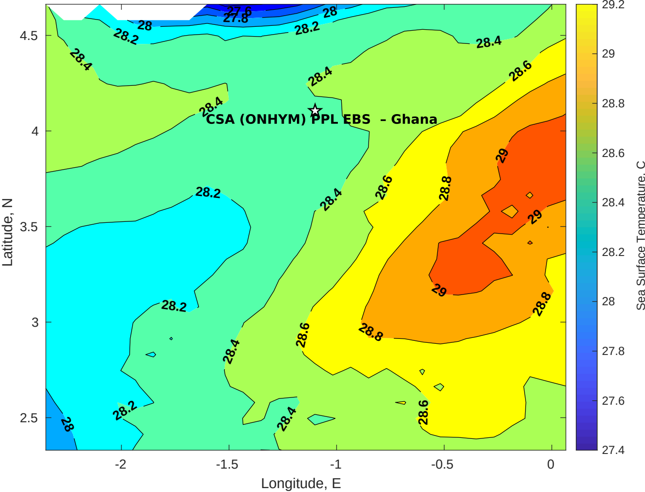
SST for CSA (ONHYM) PPL EBS - Ghana at 29-Nov-2025 00:00:00
