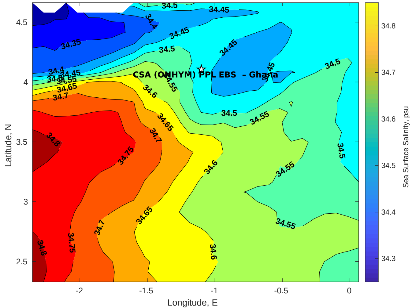
Surface Salinity for CSA (ONHYM) PPL EBS - Ghana at 29-Nov-2025 00:00:00
