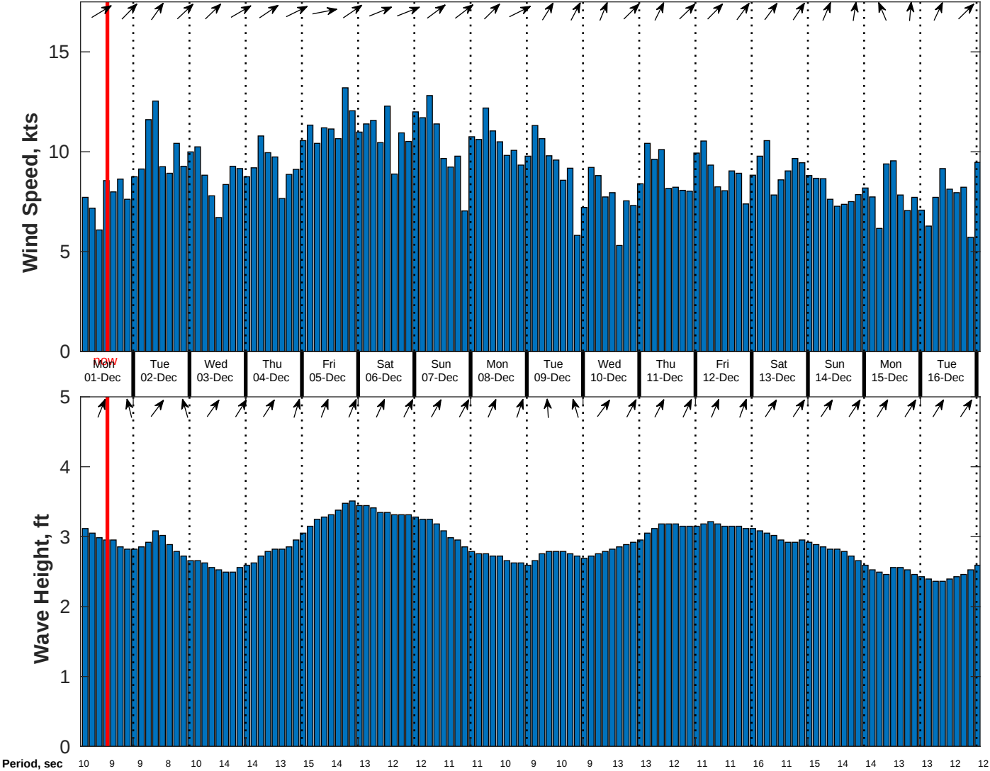
Wind & Wave Forecast for CSA (ONHYM) PPL EBS - Ghana from 30-Nov-2025 02:00:00 to 16-Dec-2025 02:00:00
