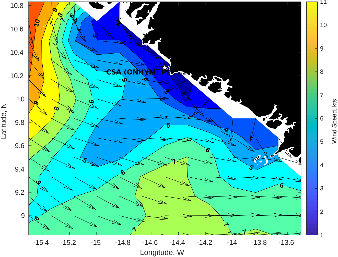
GFS Winds (kts) for CSA (ONHYM) PPL EBS - Guinea at 30-Nov-2025 09:00:00
