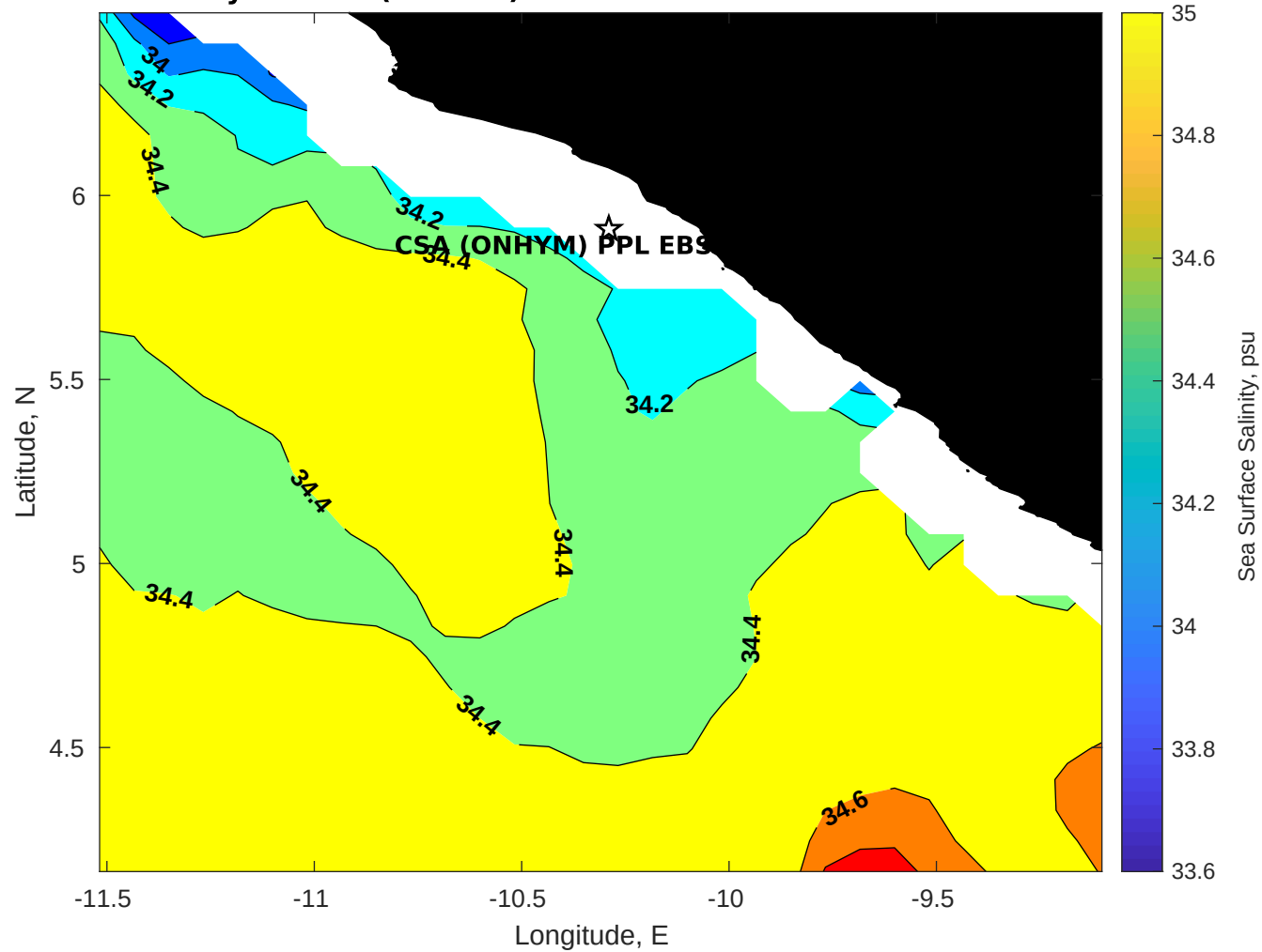
Surface Salinity for CSA (ONHYM) PPL EBS - Liberia at 29-Nov-2025 00:00:00
