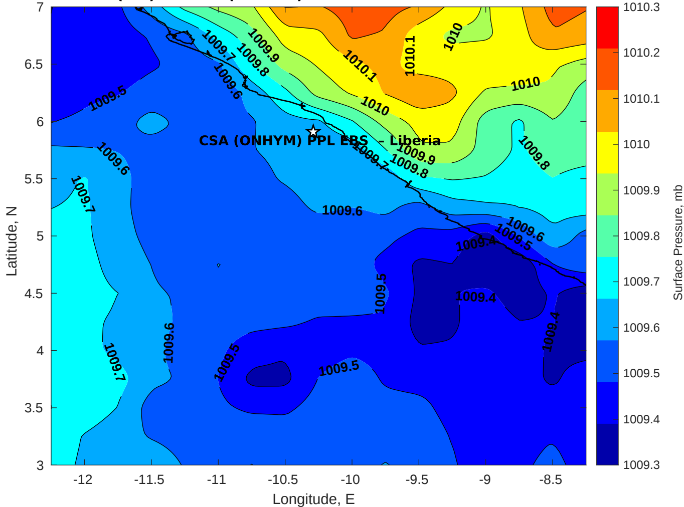
Surface Pressure (mb) for CSA (ONHYM) PPL EBS - Liberia at 01-Dec-2025 00:00:00
