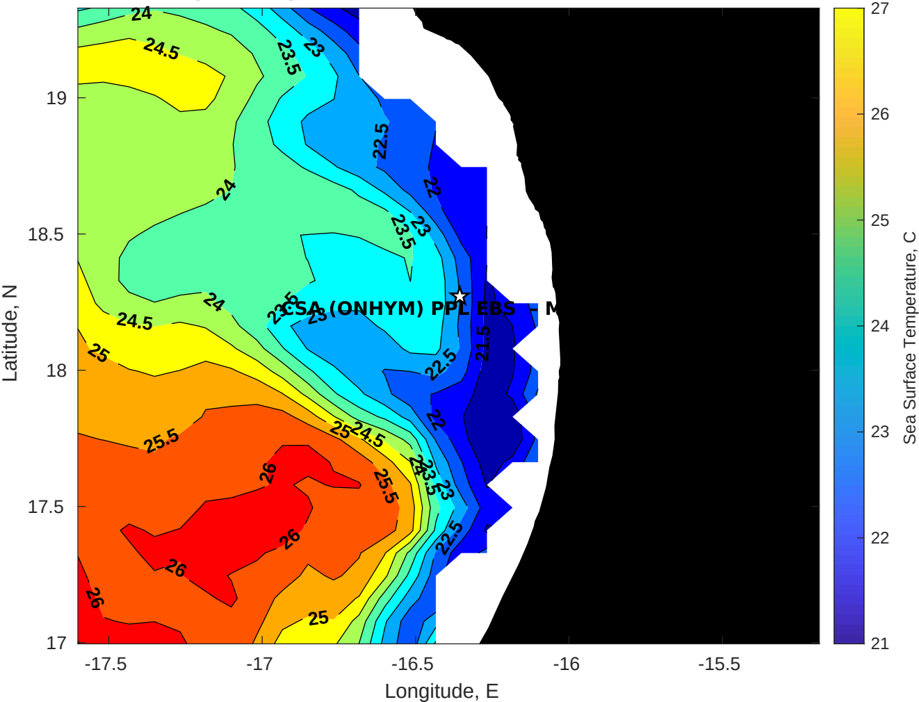
SST for CSA (ONHYM) PPL EBS - Mauritania at 29-Nov-2025 00:00:00
