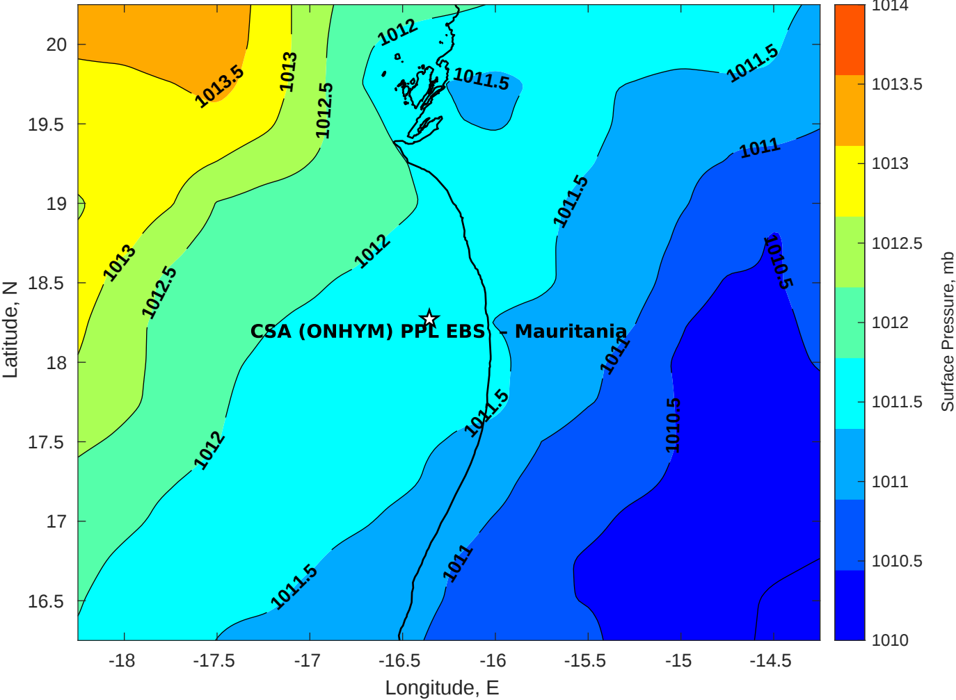
Surface Pressure (mb) for CSA (ONHYM) PPL EBS - Mauritania at 30-Nov-2025 00:00:00
