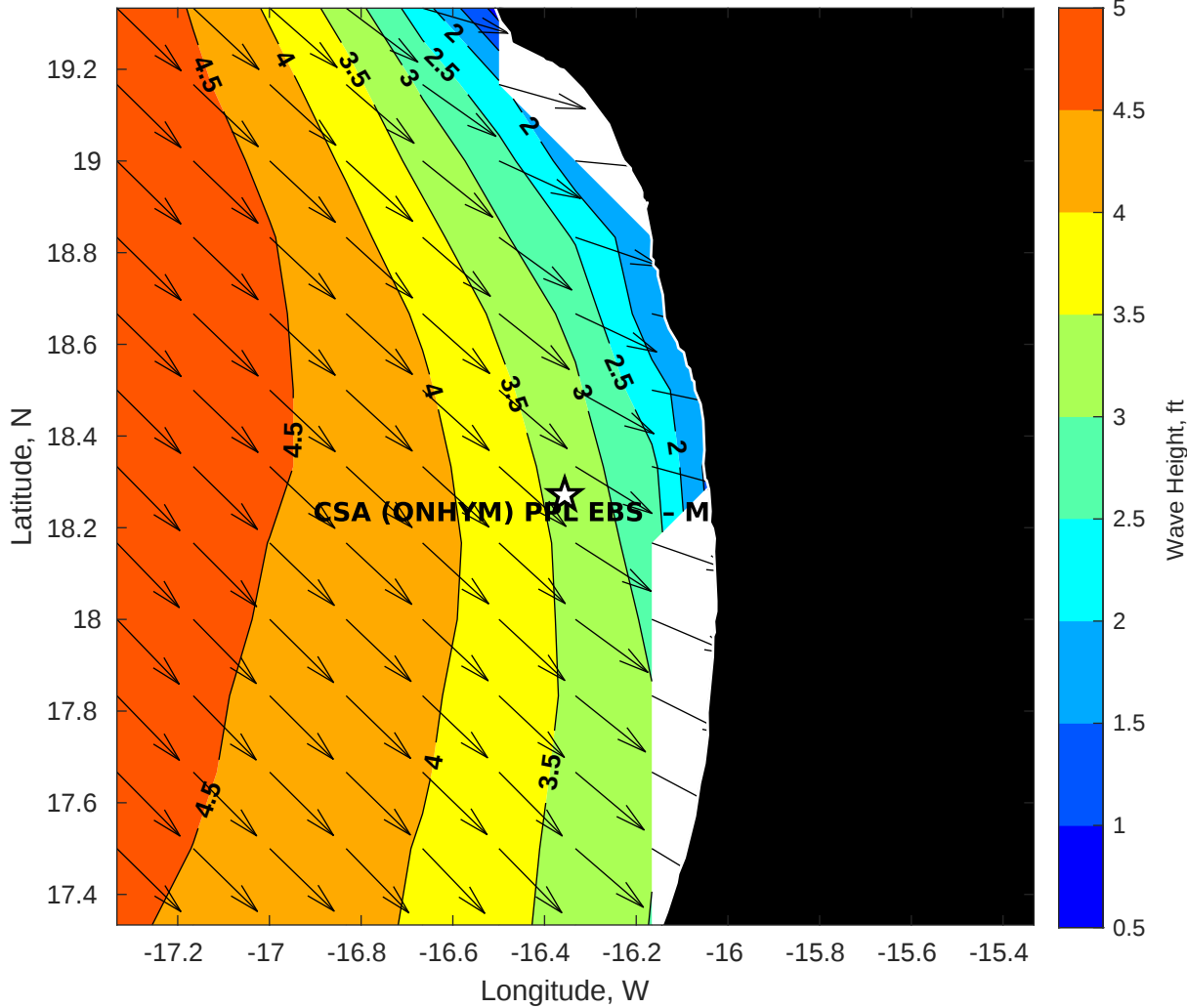
GFS Wave Height (ft) for CSA (ONHYM) PPL EBS - Mauritania at 30-Nov-2025 09:00:00
