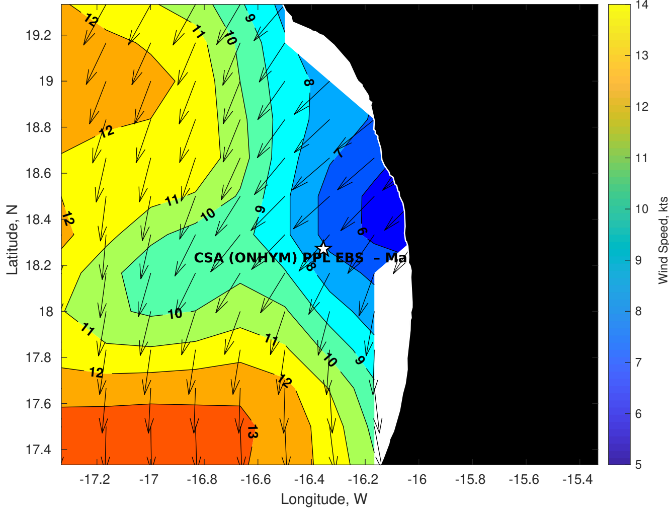
GFS Winds (kts) for CSA (ONHYM) PPL EBS - Mauritania at 30-Nov-2025 09:00:00
