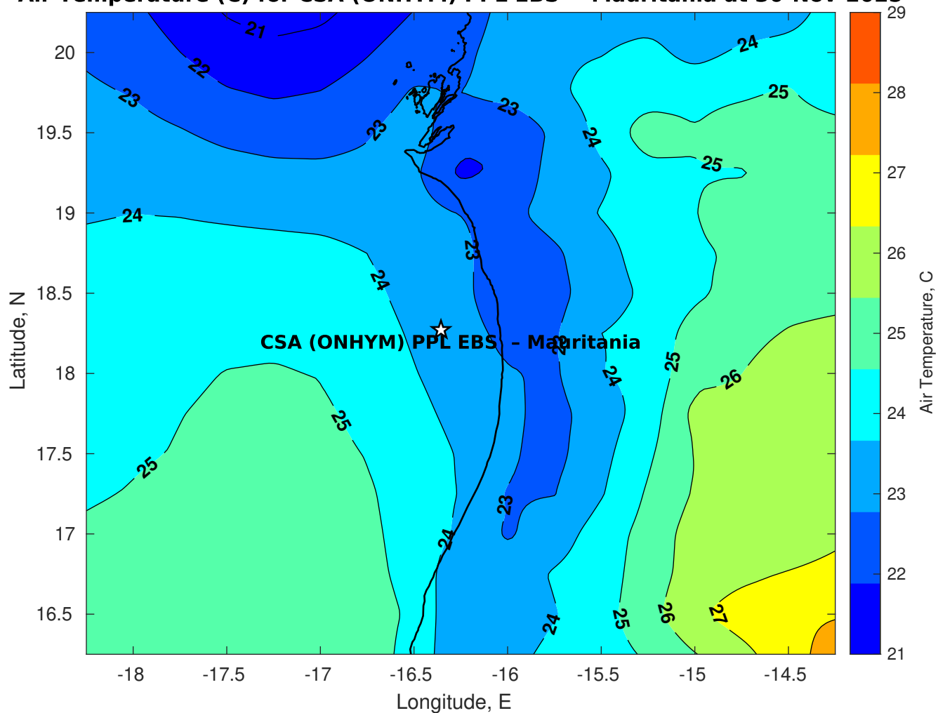
Air Temperature (C) for CSA (ONHYM) PPL EBS - Mauritania at 30-Nov-2025
