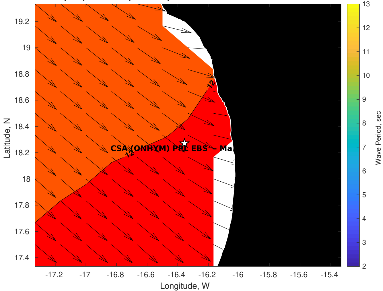
GFS Wave Period (sec) for CSA (ONHYM) PPL EBS - Mauritania at 30-Nov-2025 09:00:00
