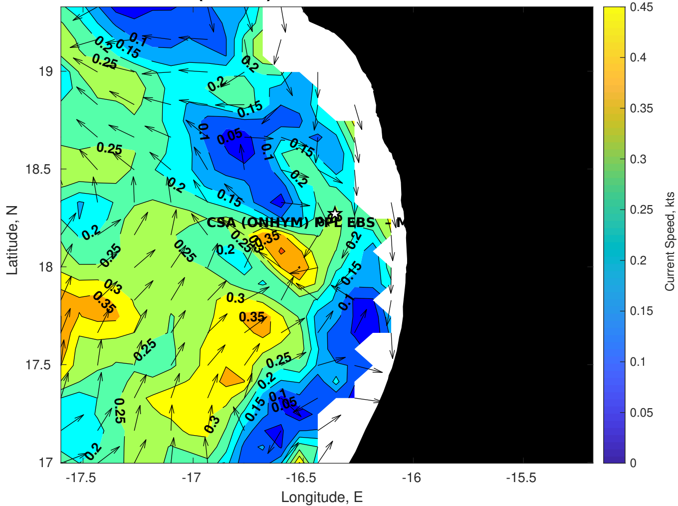
Surface Currents for CSA (ONHYM) PPL EBS - Mauritania at 29-Nov-2025 00:00:00
