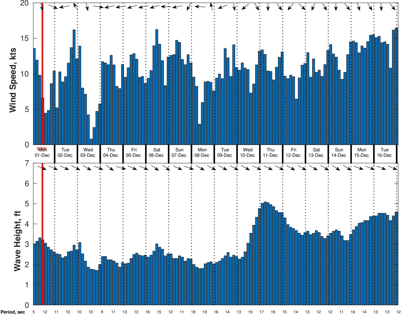
Wind & Wave Forecast for CSA (ONHYM) PPL EBS - Mauritania from 30-Nov-2025 01:00:00 to 16-Dec-2025 01:00:00
