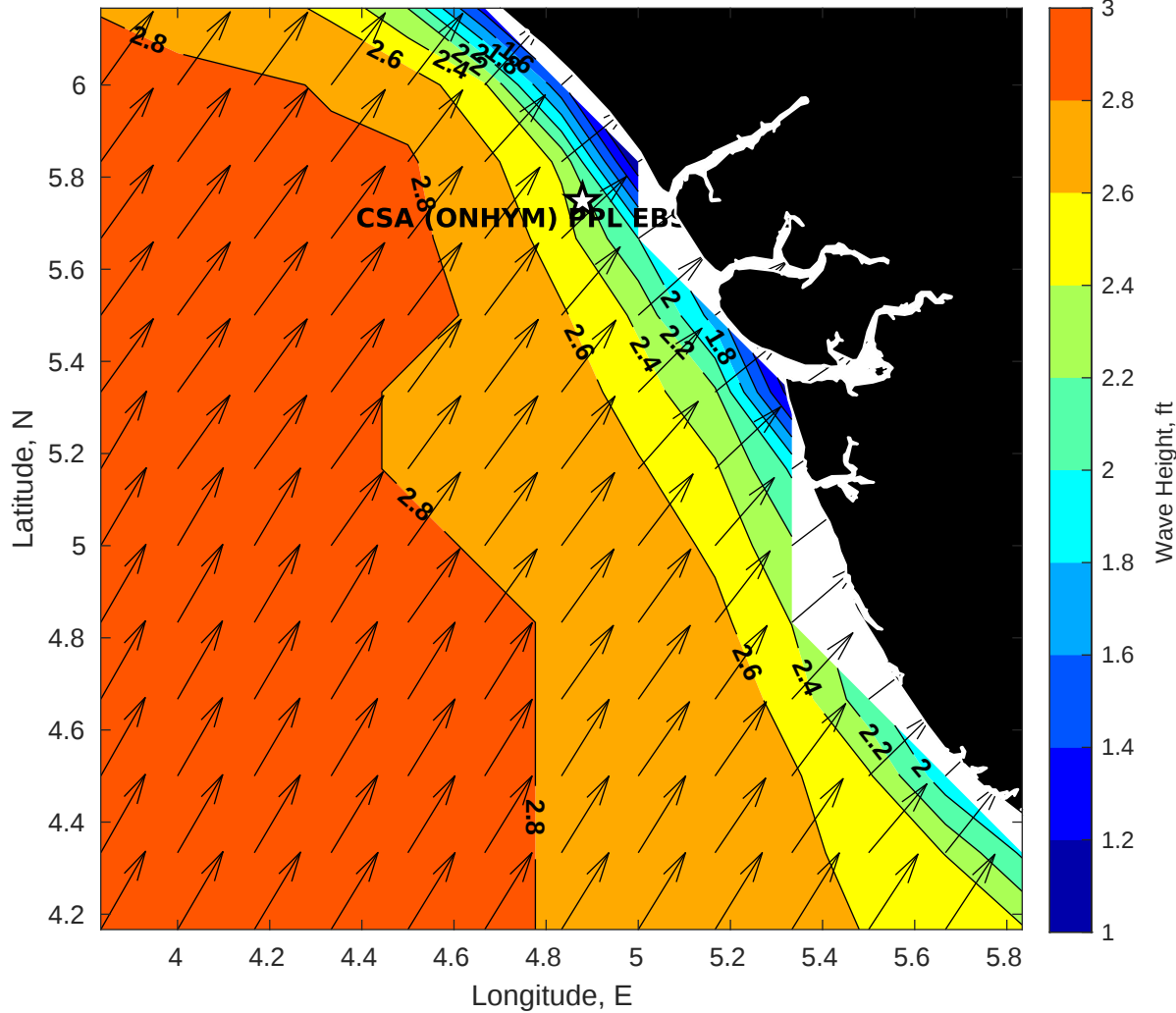
GFS Wave Height (ft) for CSA (ONHYM) PPL EBS - Nigeria at 30-Nov-2025 09:00:00
