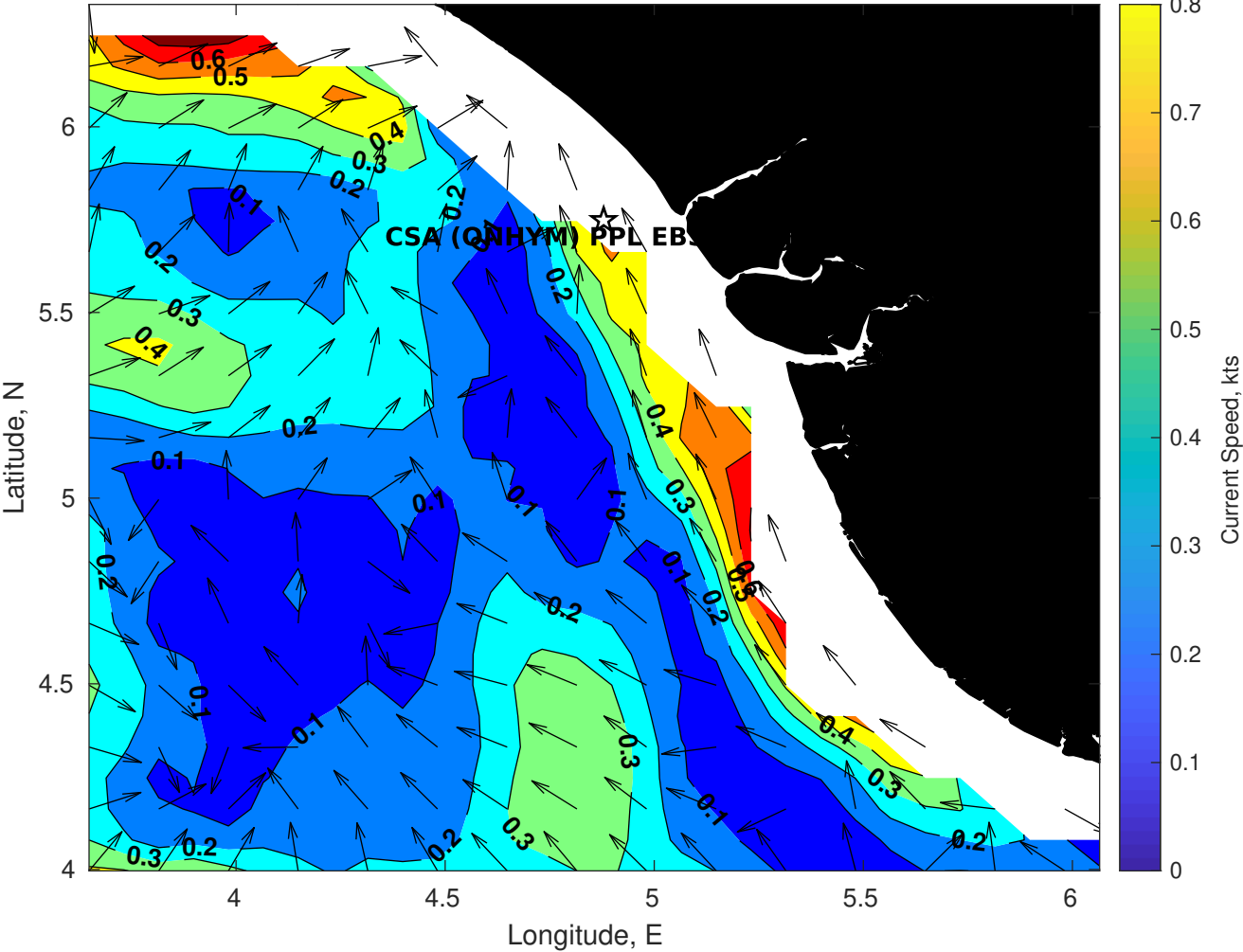
Surface Currents for CSA (ONHYM) PPL EBS - Nigeria at 29-Nov-2025 00:00:00
