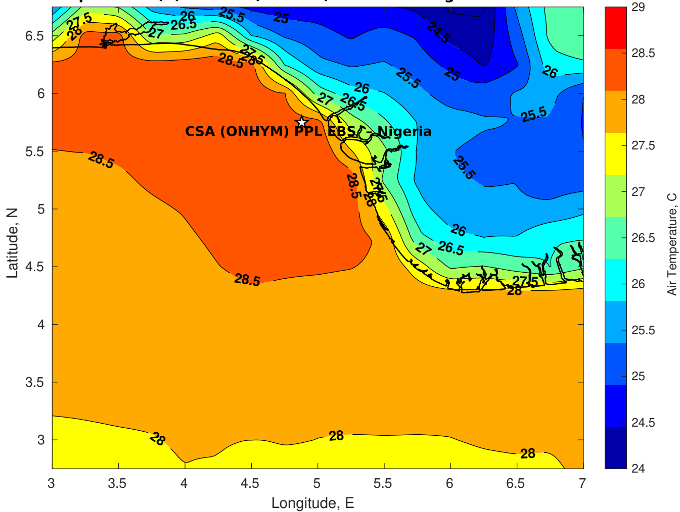
Air Temperature (C) for CSA (ONHYM) PPL EBS - Nigeria at 30-Nov-2025
