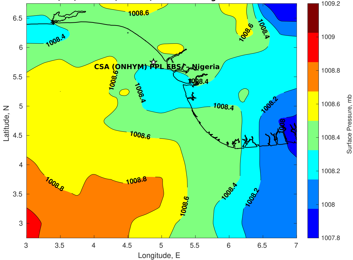
Surface Pressure (mb) for CSA (ONHYM) PPL EBS - Nigeria at 30-Nov-2025 00:00:00
