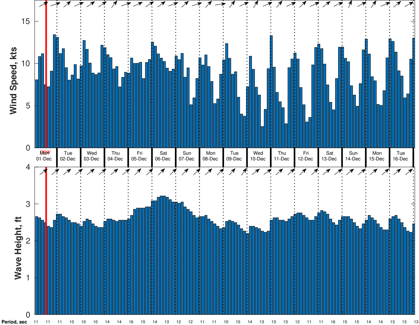
Wind & Wave Forecast for CSA (ONHYM) PPL EBS - Nigeria from 30-Nov-2025 02:00:00 to 16-Dec-2025 02:00:00
