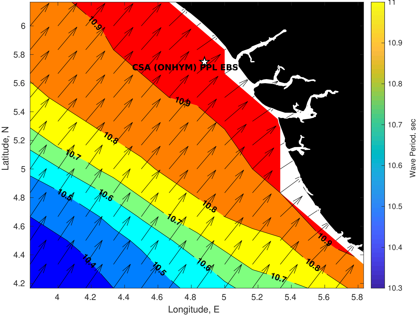
GFS Wave Period (sec) for CSA (ONHYM) PPL EBS - Nigeria at 30-Nov-2025 09:00:00
