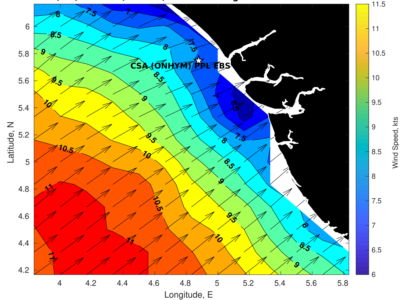
GFS Winds (kts) for CSA (ONHYM) PPL EBS - Nigeria at 30-Nov-2025 09:00:00
