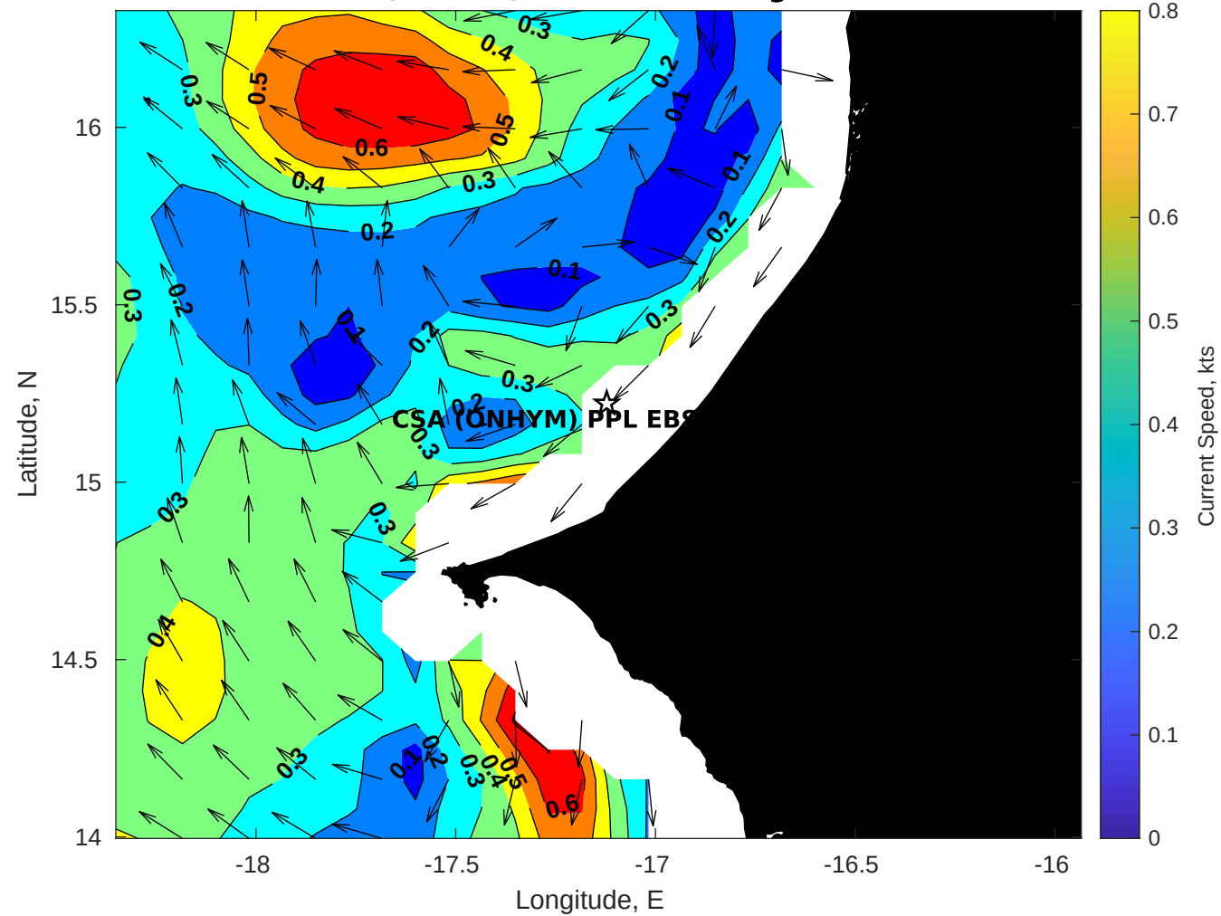
Surface Currents for CSA (ONHYM) PPL EBS - Senegal at 29-Nov-2025 00:00:00
