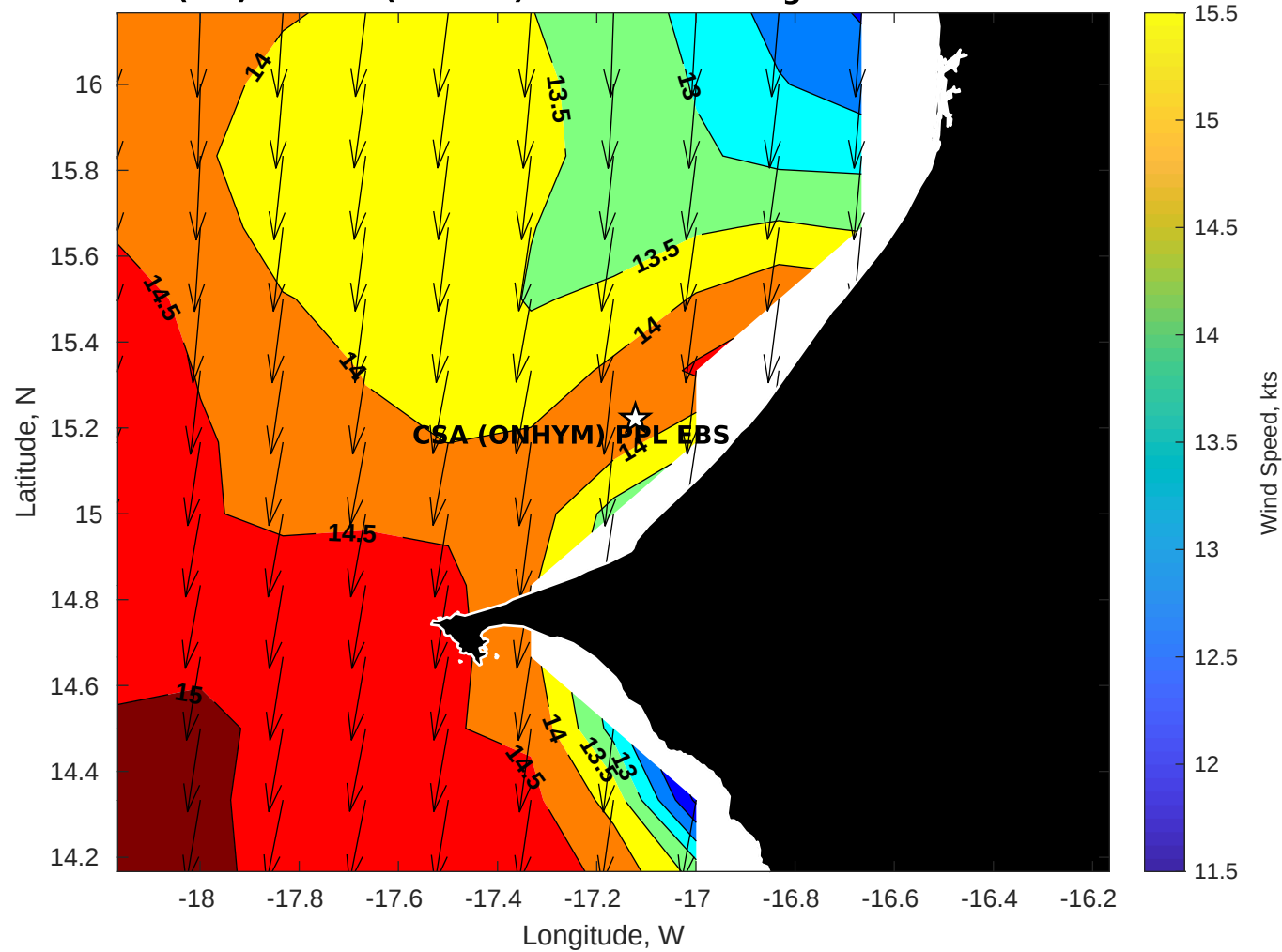
GFS Winds (kts) for CSA (ONHYM) PPL EBS - Senegal at 30-Nov-2025 09:00:00
