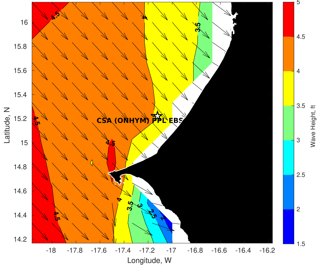
GFS Wave Height (ft) for CSA (ONHYM) PPL EBS - Senegal at 30-Nov-2025 09:00:00
