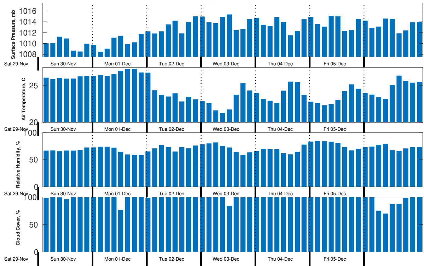
Met Forecast for CSA (ONHYM) PPL EBS - Senegal from 30-Nov-2025 00:00:00 to 07-Dec-2025 00:00:00
