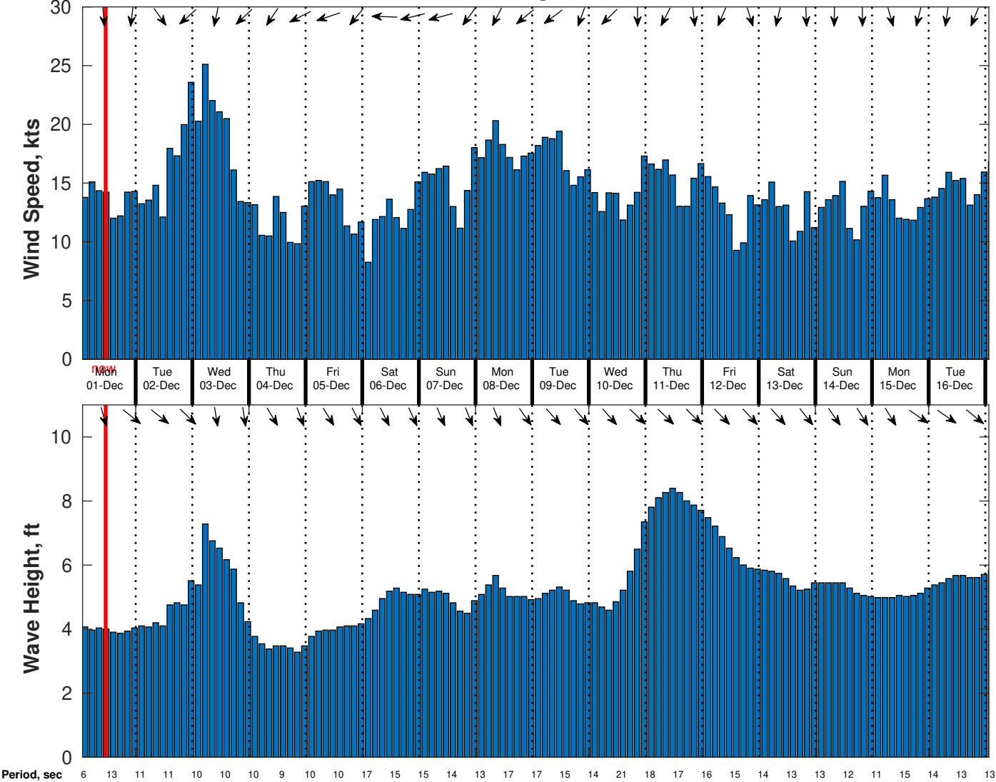
Wind & Wave Forecast for CSA (ONHYM) PPL EBS - Senegal from 30-Nov-2025 01:00:00 to 16-Dec-2025 01:00:00
