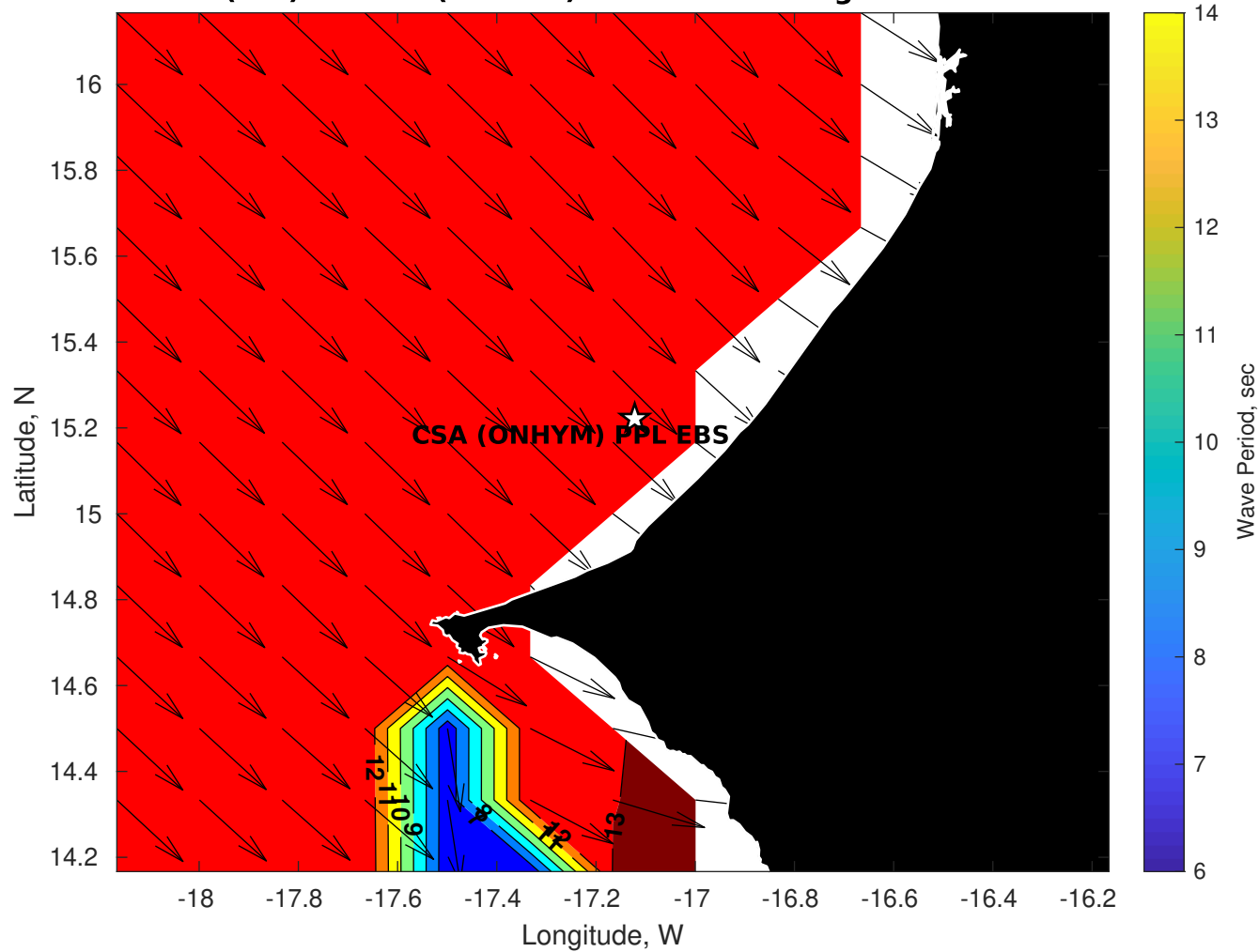
GFS Wave Period (sec) for CSA (ONHYM) PPL EBS - Senegal at 30-Nov-2025 09:00:00
