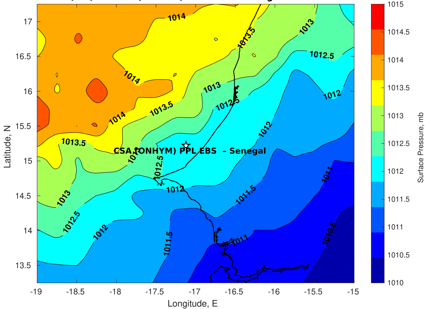
Surface Pressure (mb) for CSA (ONHYM) PPL EBS - Senegal at 02-Dec-2025 00:00:00
