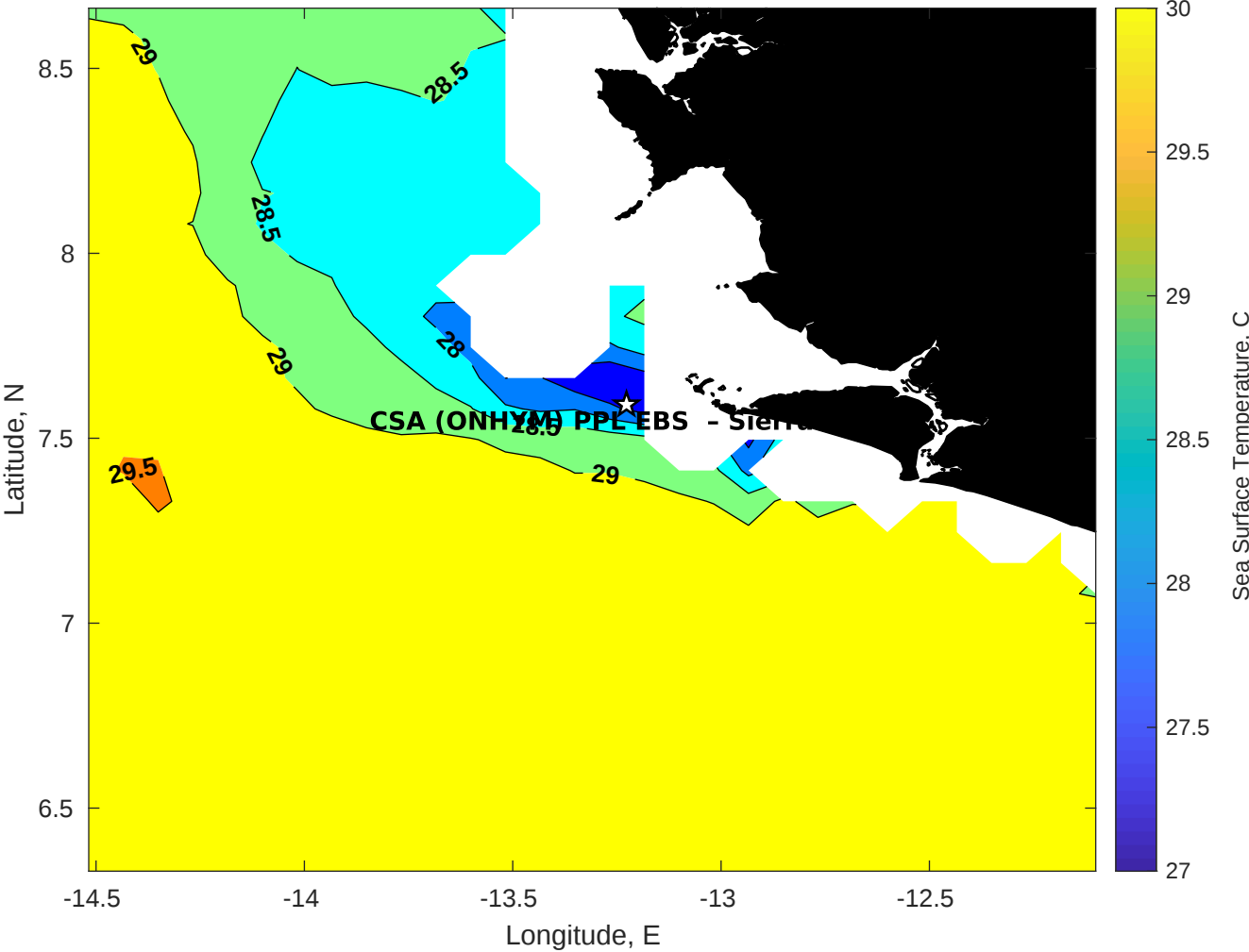
SST for CSA (ONHYM) PPL EBS - Sierra Leone at 29-Nov-2025 00:00:00
