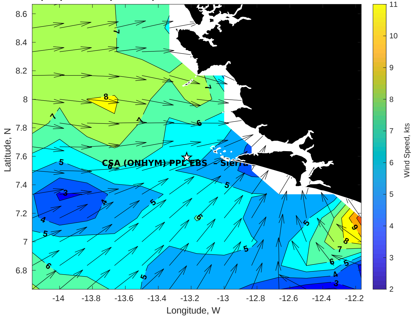
GFS Winds (kts) for CSA (ONHYM) PPL EBS - Sierra Leone at 30-Nov-2025 09:00:00
