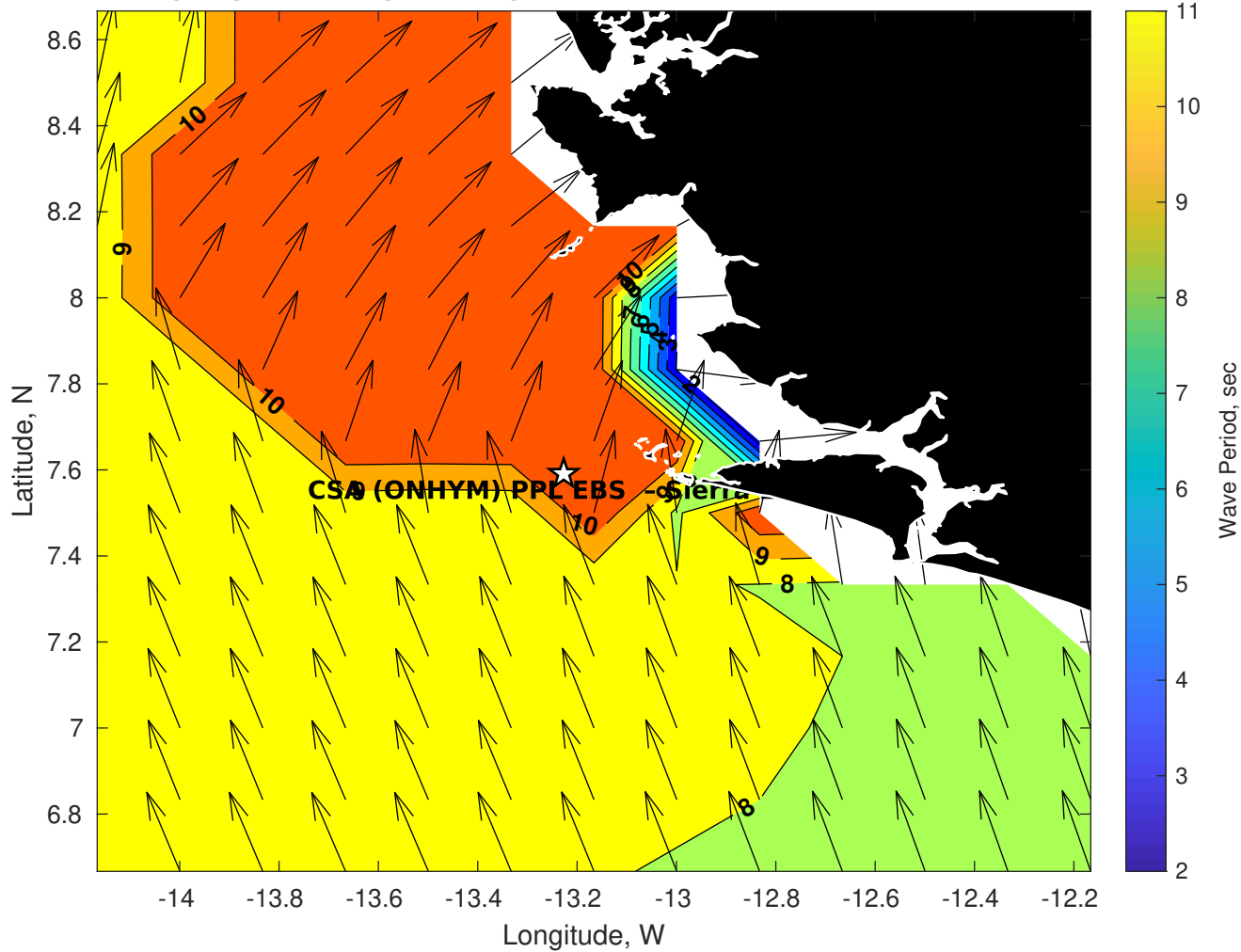
GFS Wave Period (sec) for CSA (ONHYM) PPL EBS - Sierra Leone at 30-Nov-2025 09:00:00
