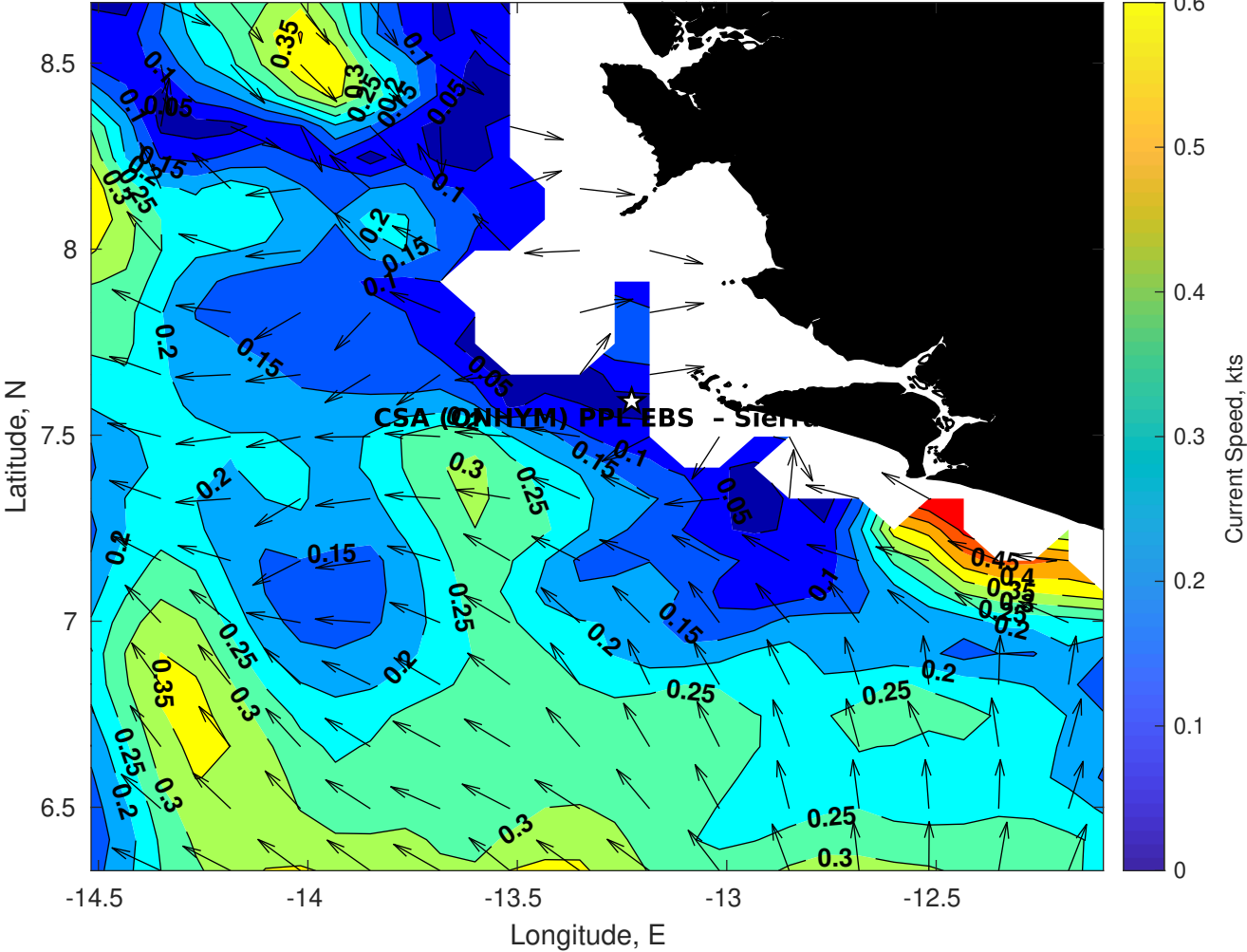
Surface Currents for CSA (ONHYM) PPL EBS - Sierra Leone at 29-Nov-2025 00:00:00
