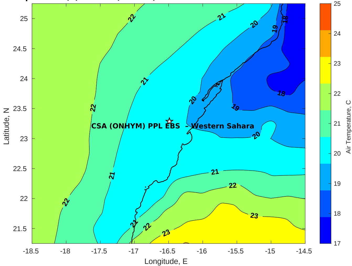
Air Temperature (C) for CSA (ONHYM) PPL EBS - Western Sahara at 30-Nov-2025
