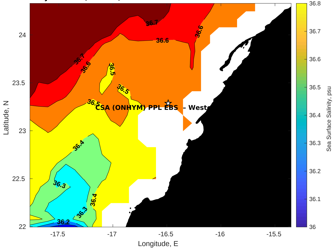
Surface Salinity for CSA (ONHYM) PPL EBS - Western Sahara at 29-Nov-2025 00:00:00
