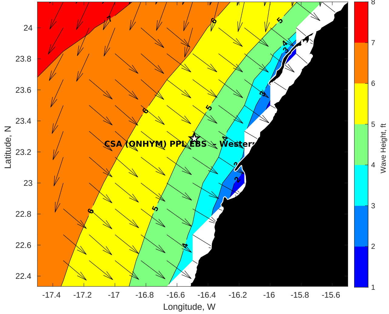
GFS Wave Height (ft) for CSA (ONHYM) PPL EBS - Western Sahara at 30-Nov-2025 09:00:00
