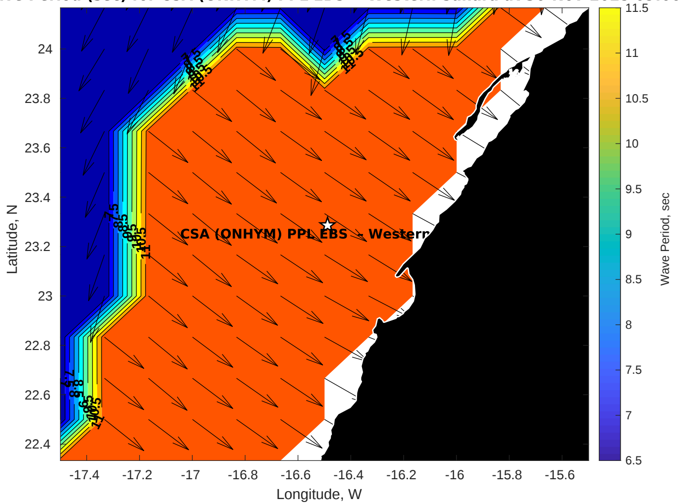
GFS Wave Period (sec) for CSA (ONHYM) PPL EBS - Western Sahara at 30-Nov-2025 09:00:00
