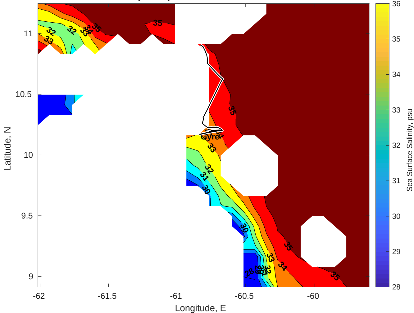
Surface Salinity for Gyre at 29-Nov-2025 00:00:00
