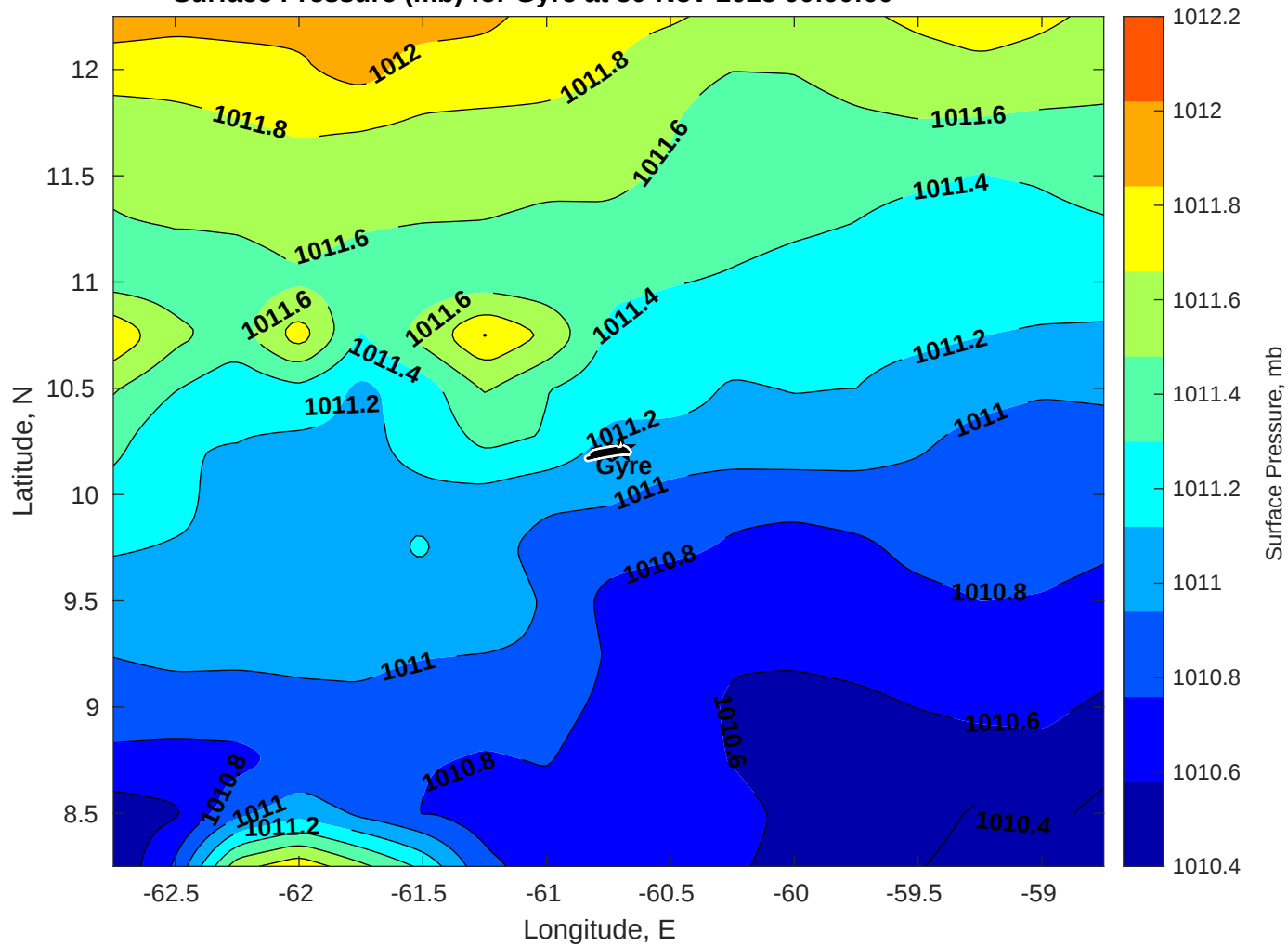
Surface Pressure (mb) for Gyre at 30-Nov-2025 00:00:00
