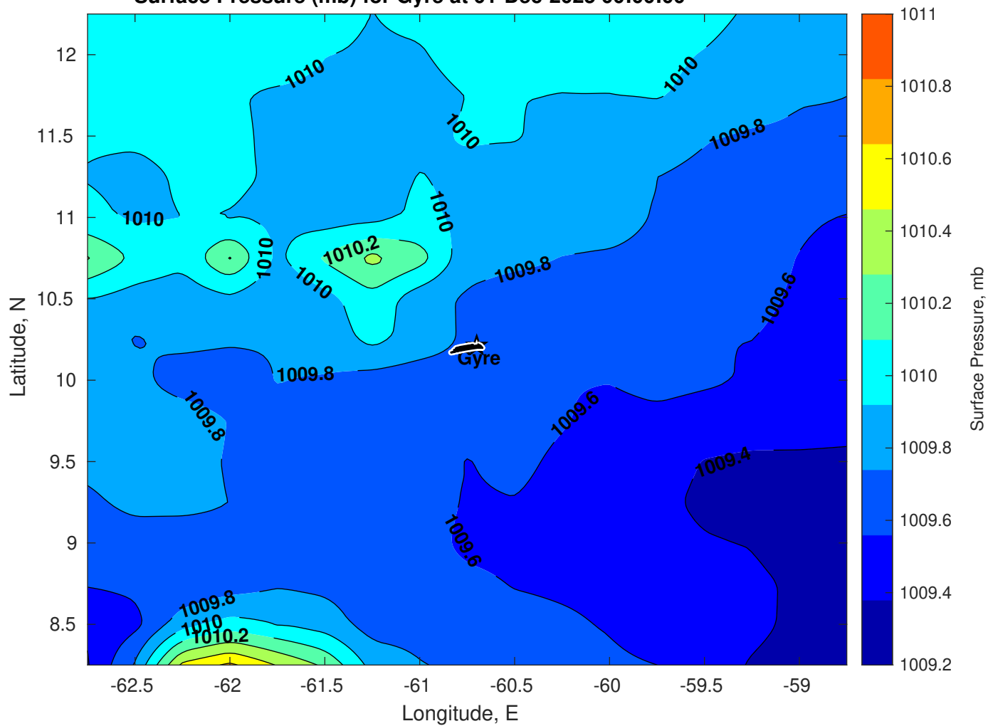
Surface Pressure (mb) for Gyre at 01-Dec-2025 00:00:00
