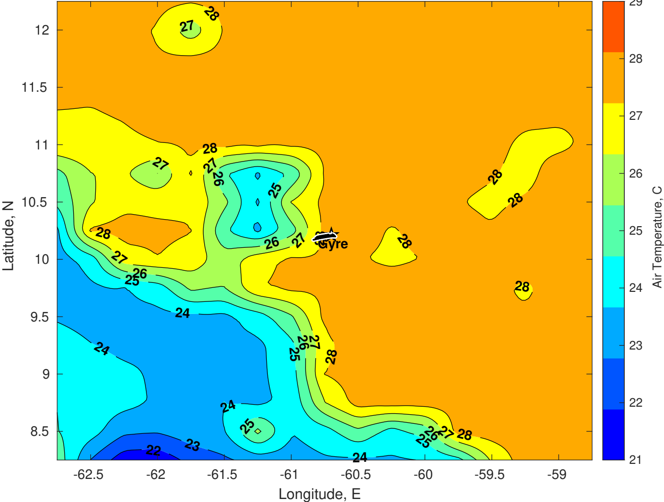
Air Temperature (C) for Gyre at 30-Nov-2025
