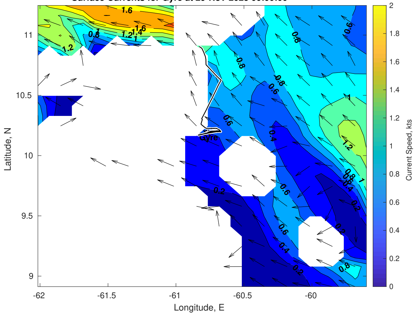
Surface Currents for Gyre at 29-Nov-2025 00:00:00
