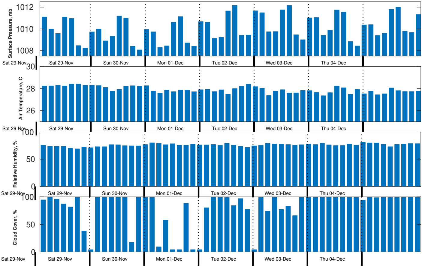
Met Forecast for Gyre from 29-Nov-2025 20:00:00 to 06-Dec-2025 20:00:00
