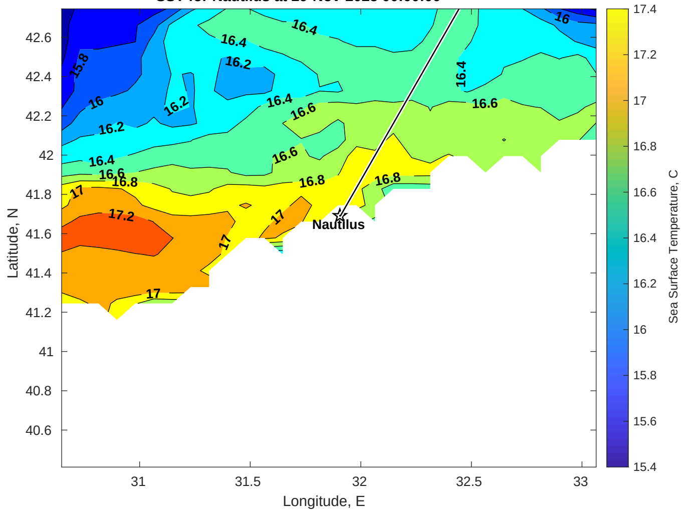
SST for Nautilus at 29-Nov-2025 00:00:00
