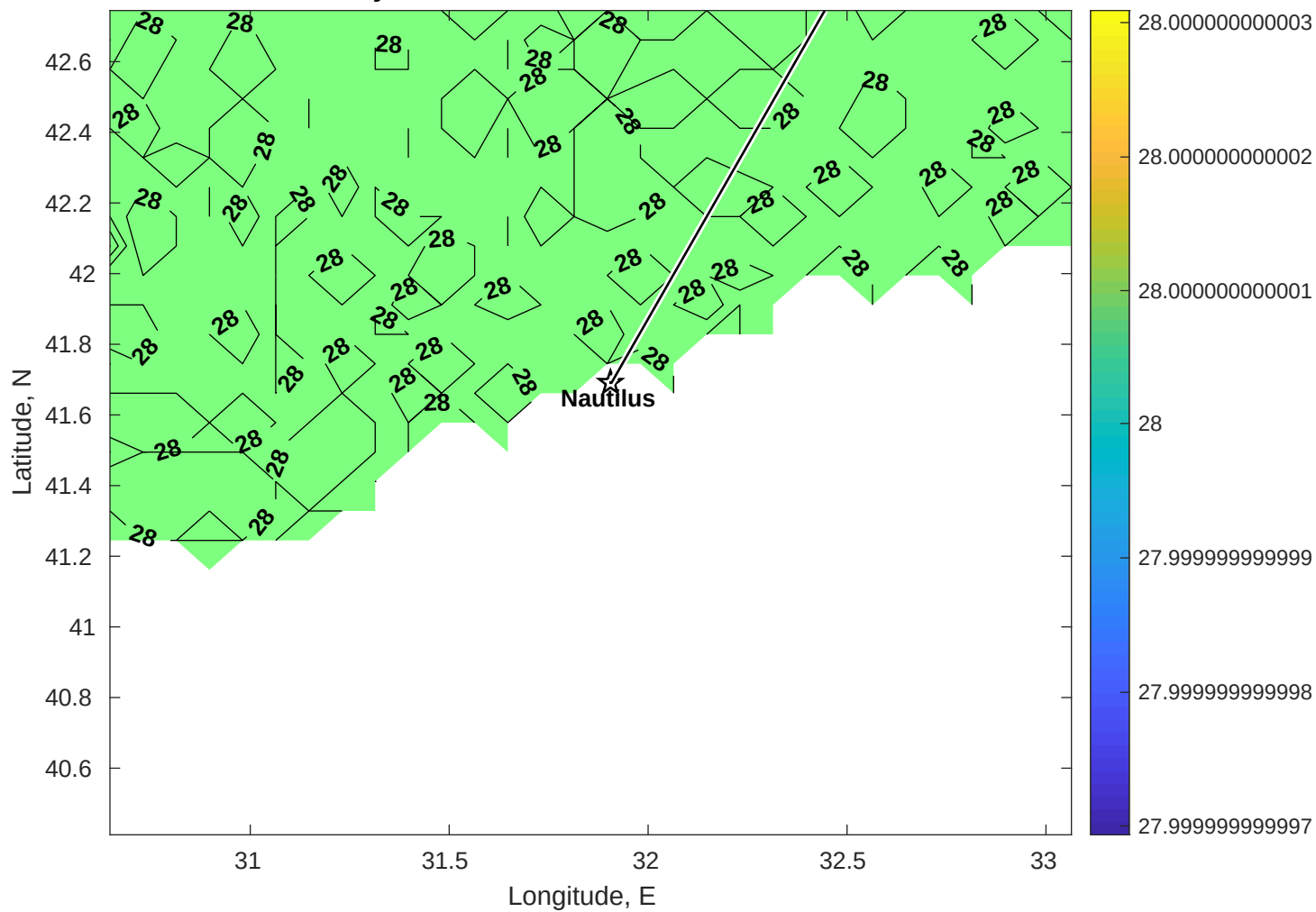
Surface Salinity for Nautilus at 29-Nov-2025 00:00:00
