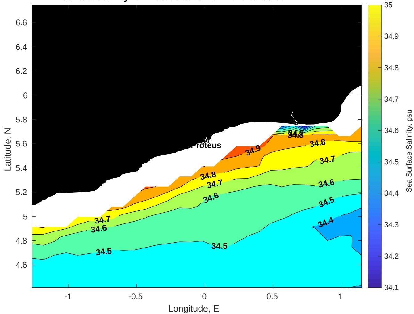
Surface Salinity for Proteus at 29-Nov-2025 00:00:00
