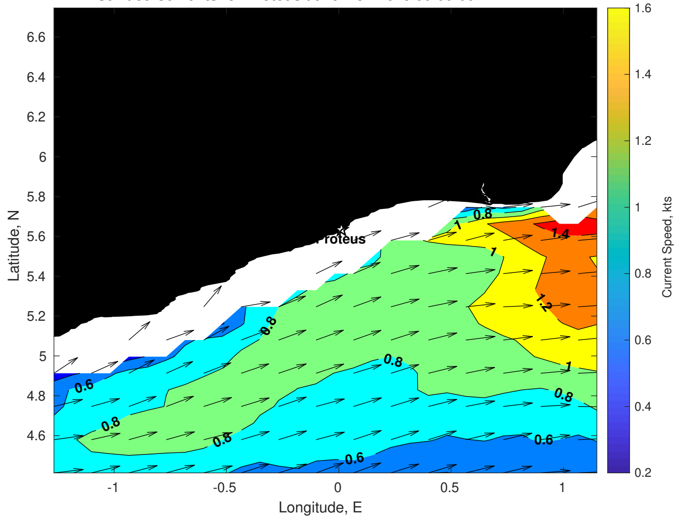
Surface Currents for Proteus at 29-Nov-2025 00:00:00
