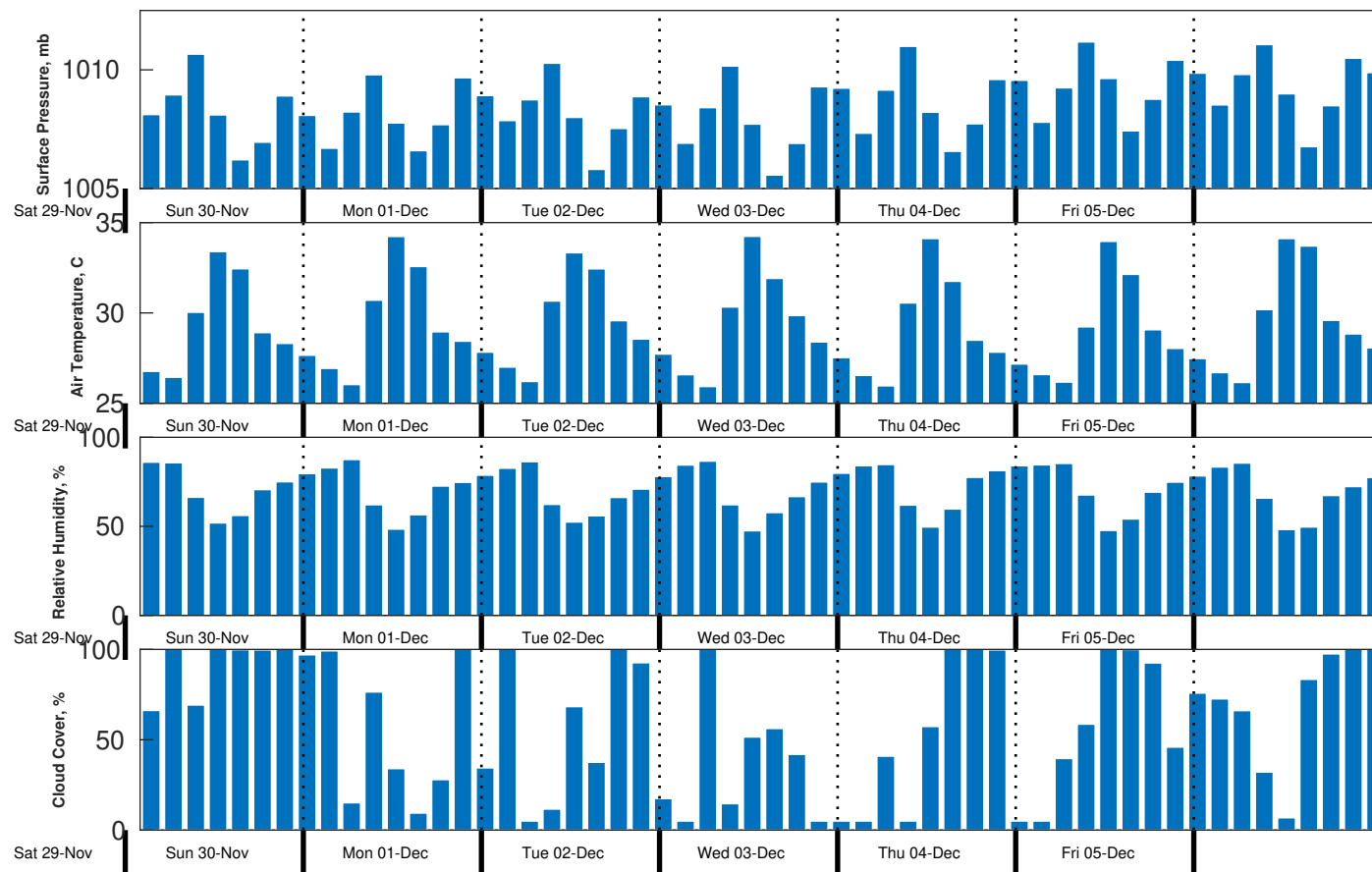
Met Forecast for Proteus from 30-Nov-2025 00:00:00 to 07-Dec-2025 00:00:00
