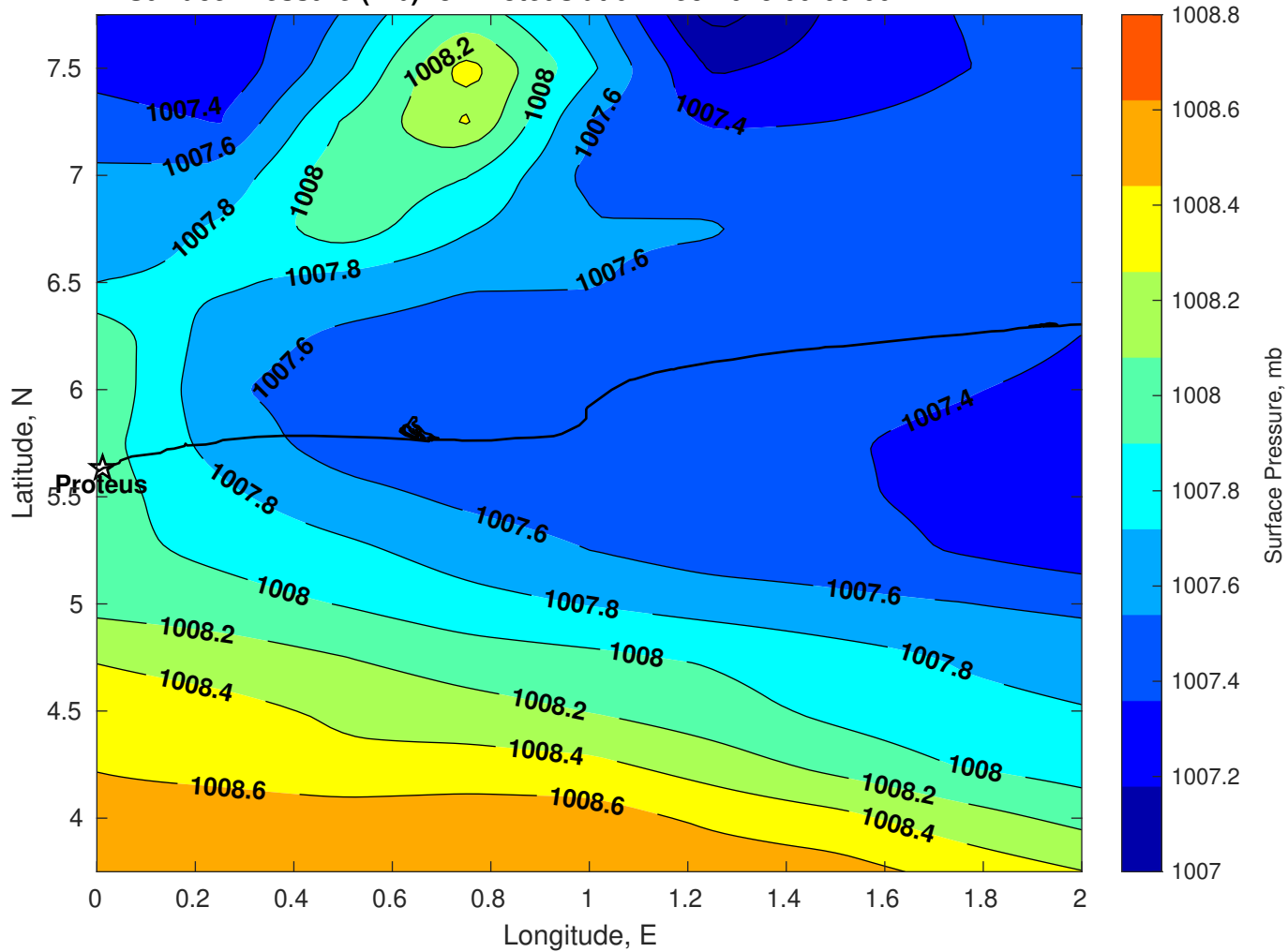
Surface Pressure (mb) for Proteus at 01-Dec-2025 00:00:00
