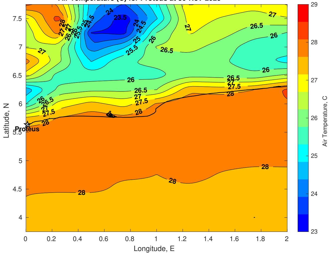
Air Temperature (C) for Proteus at 30-Nov-2025
