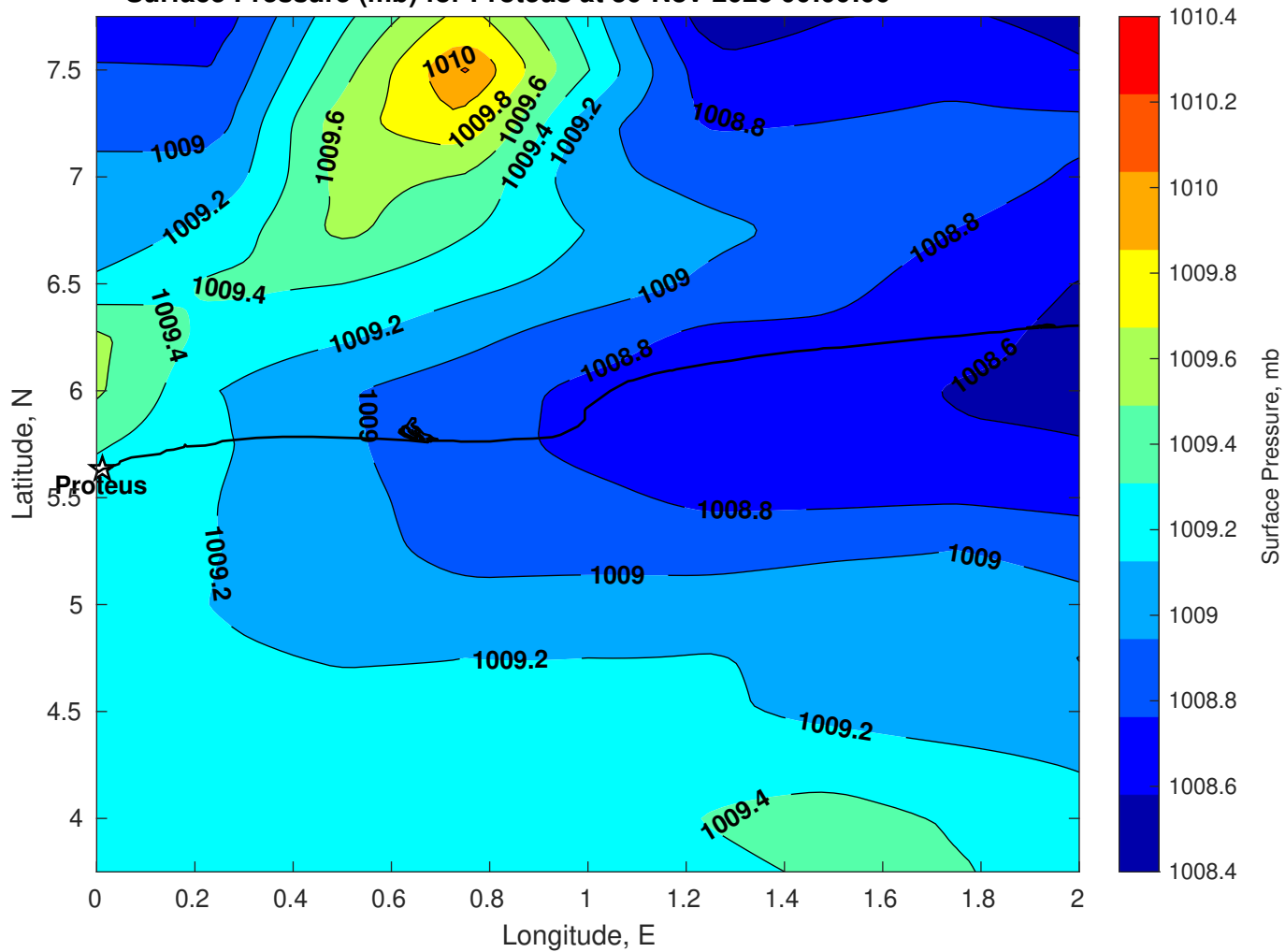
Surface Pressure (mb) for Proteus at 30-Nov-2025 00:00:00
