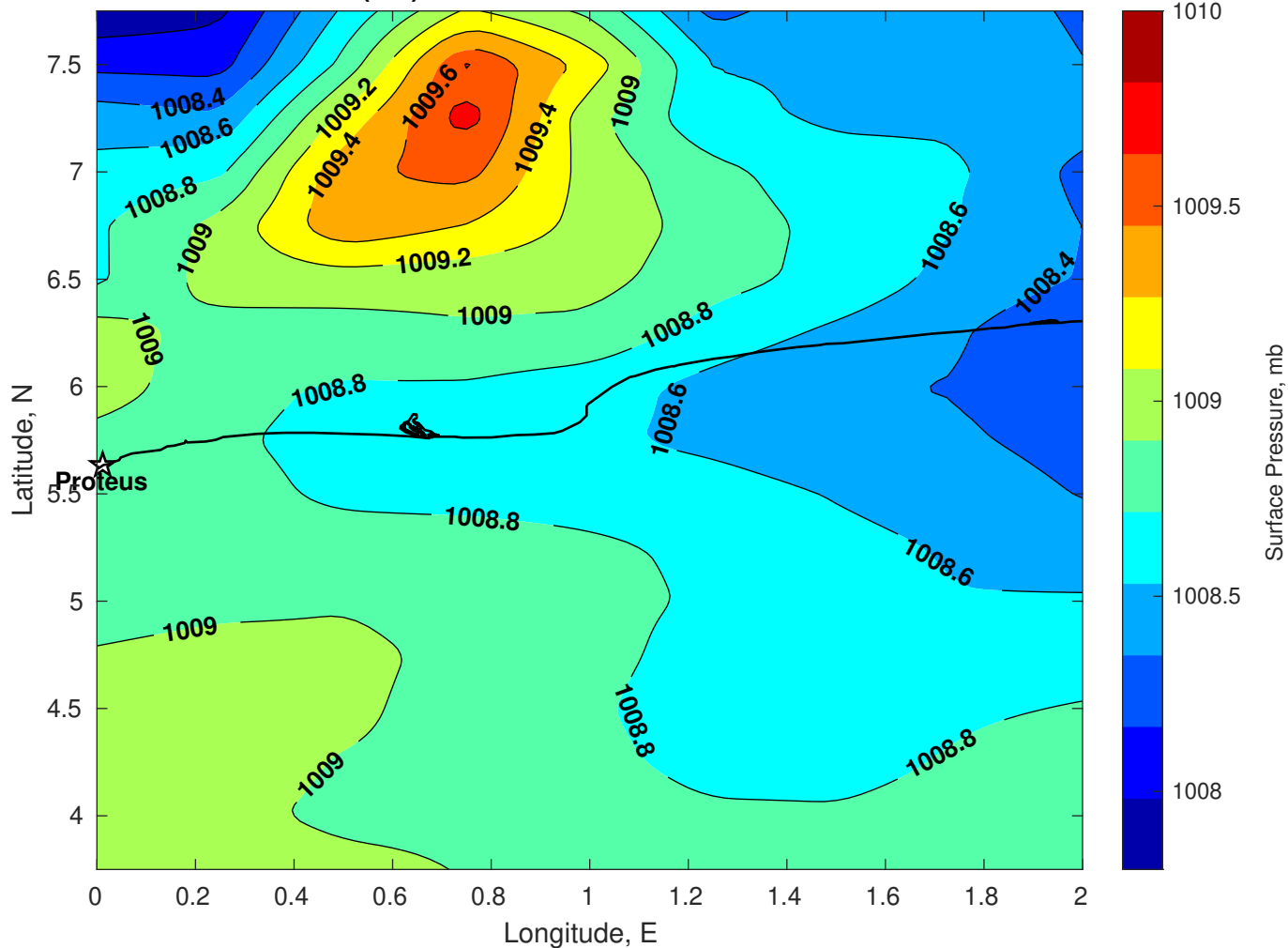
Surface Pressure (mb) for Proteus at 02-Dec-2025 00:00:00
