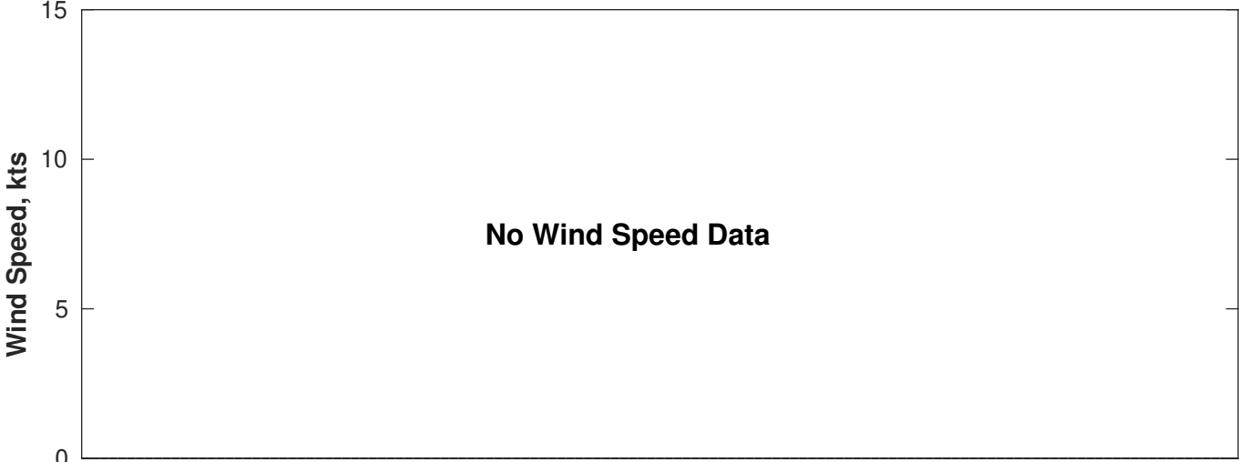
Wind & Wave Forecast for Proteus from 30-Nov-2025 01:00:00 to 16-Dec-2025 01:00:00
