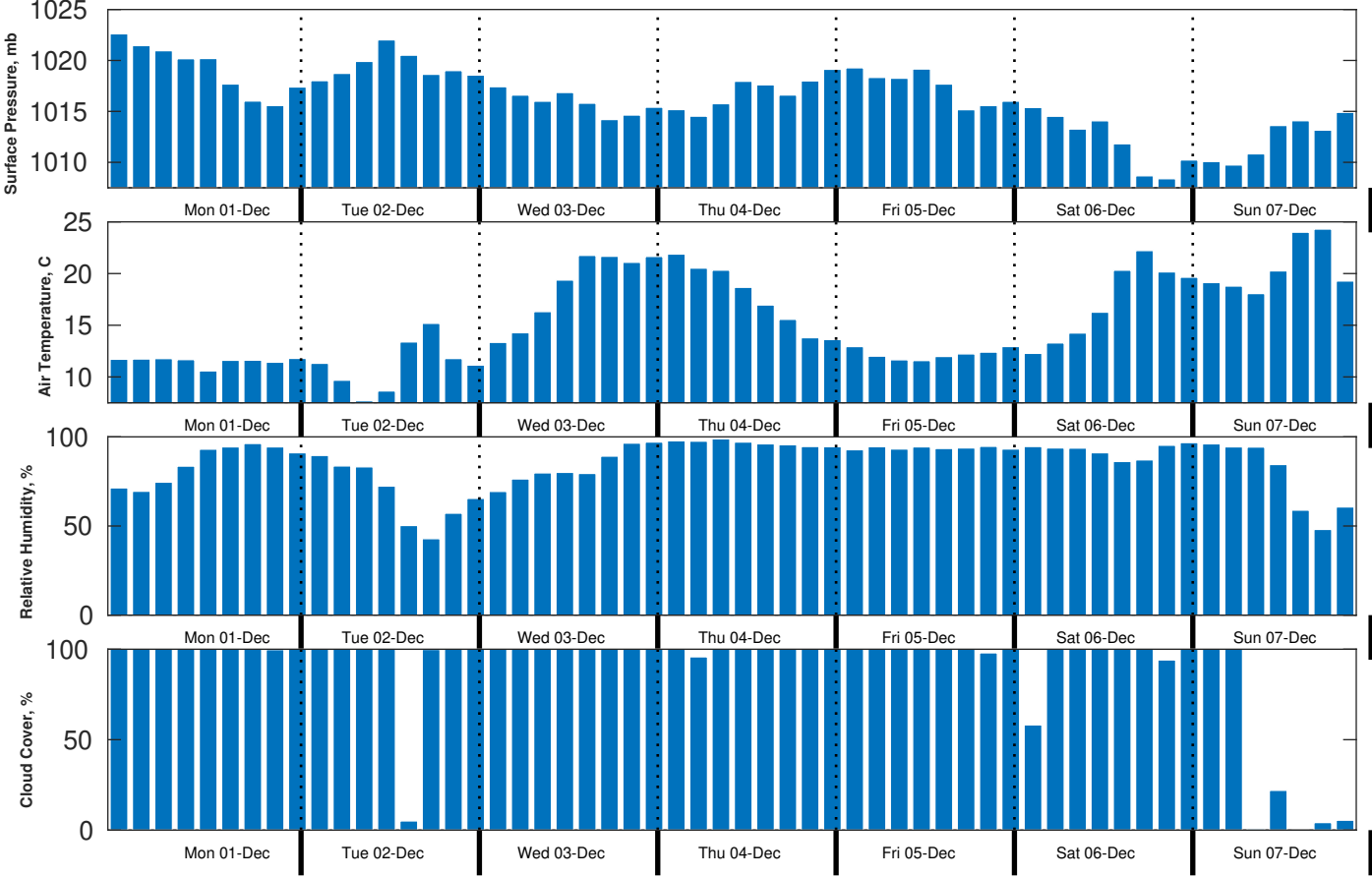
Met Forecast for Brooks McCall from 01-Dec-2025 00:00:00 to 08-Dec-2025 00:00:00
