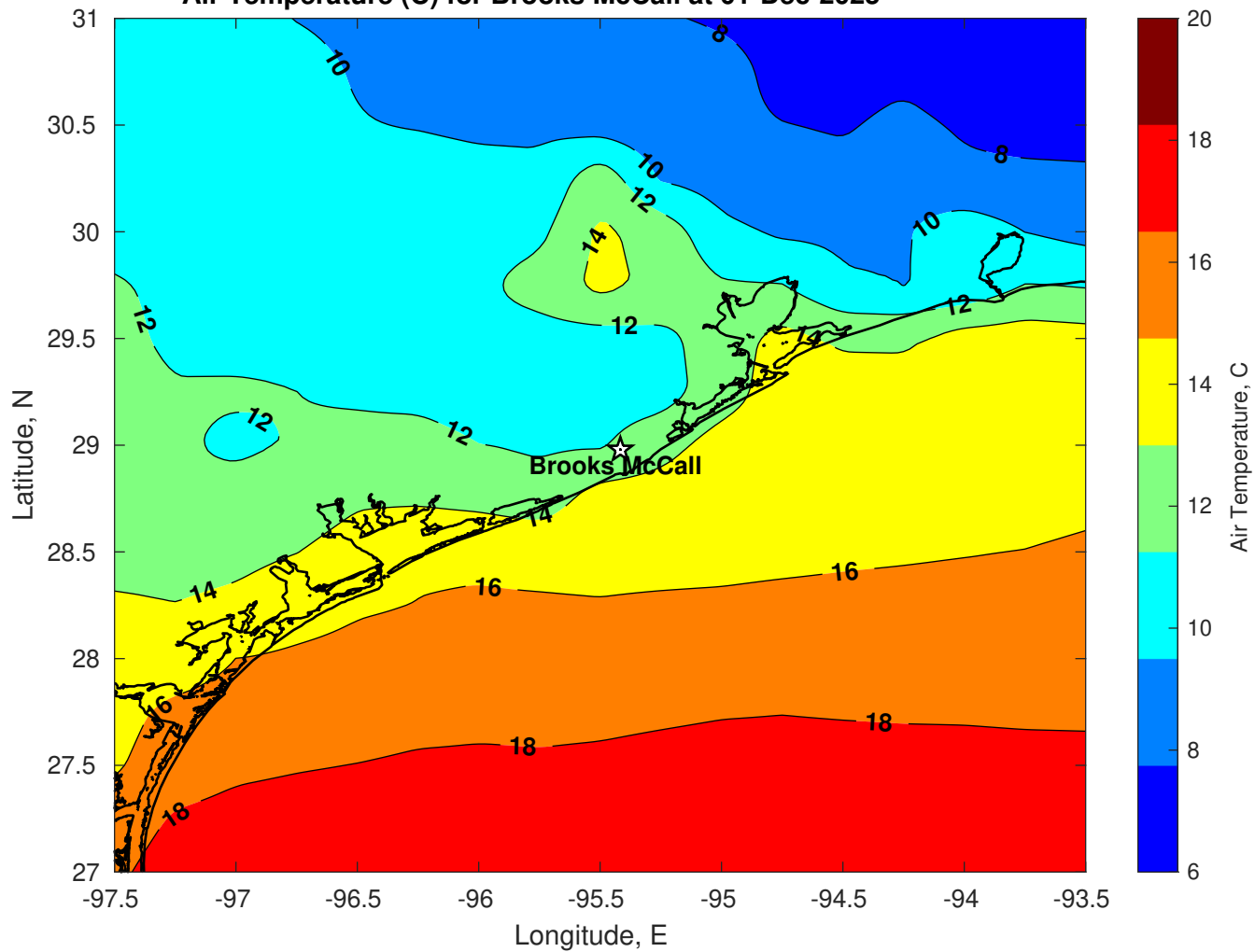
Air Temperature (C) for Brooks McCall at 01-Dec-2025
