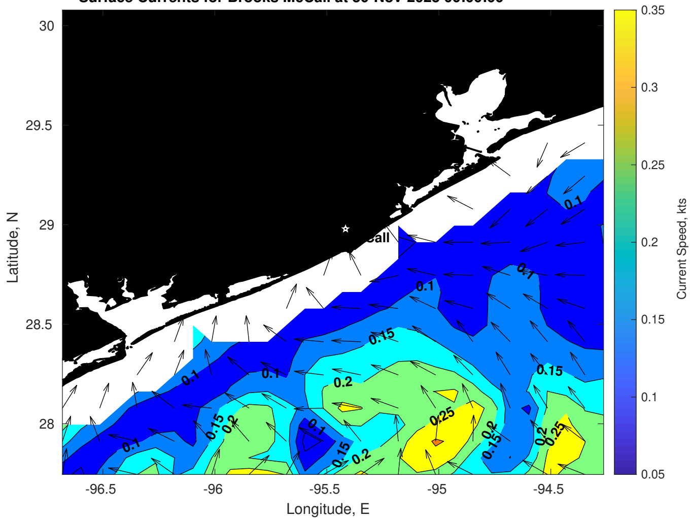
Surface Currents for Brooks McCall at 30-Nov-2025 00:00:00
