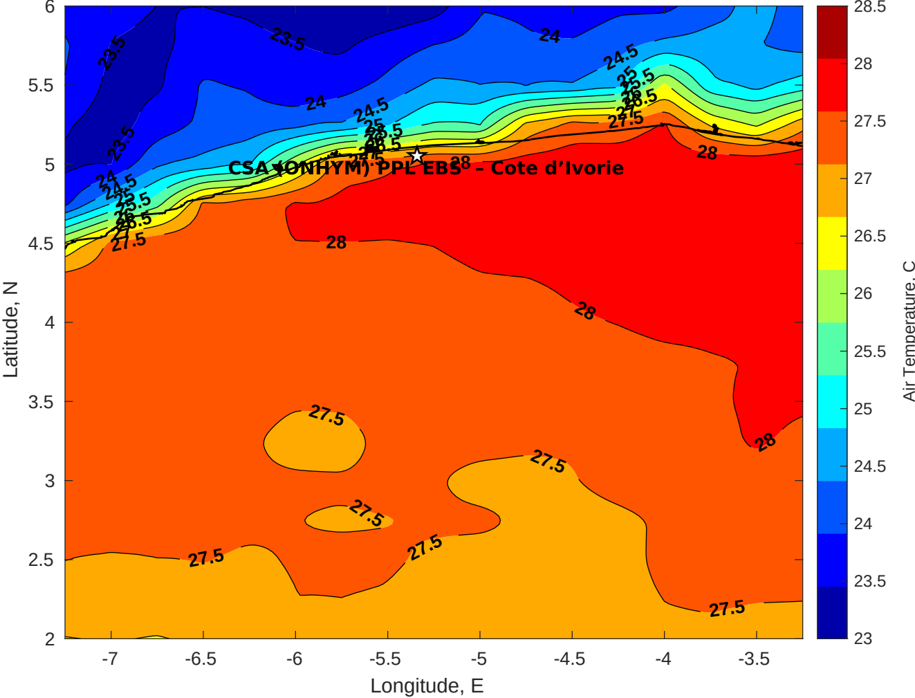
Air Temperature (C) for CSA (ONHYM) PPL EBS - Cote d'Ivoire at 01-Dec-2025
