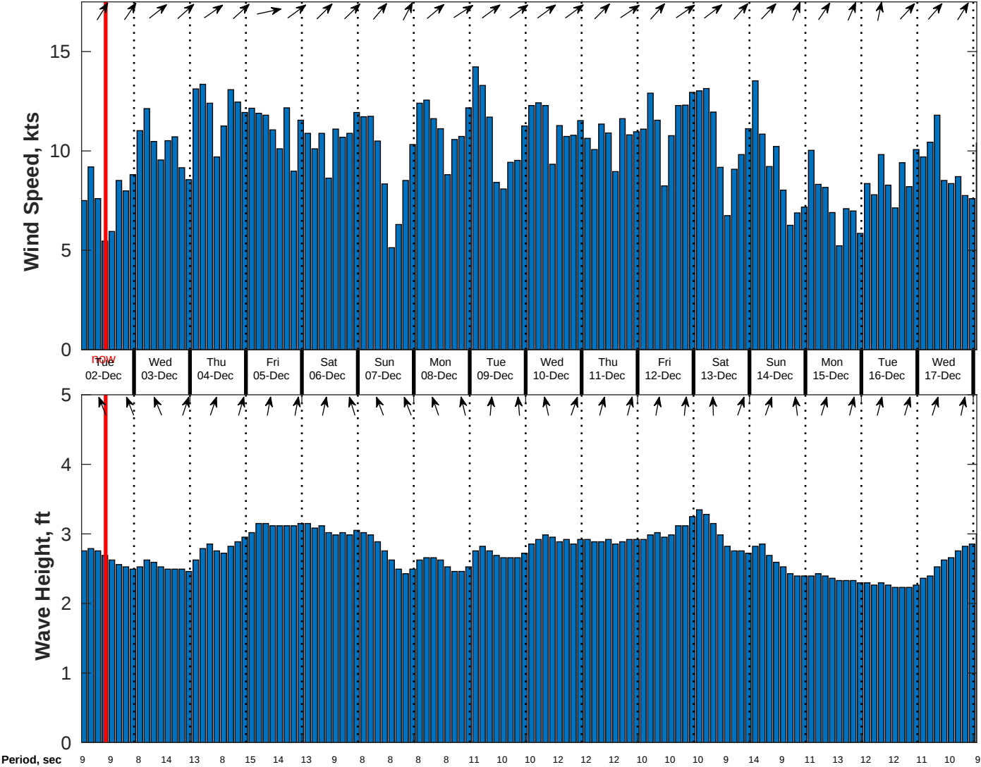
Wind & Wave Forecast for CSA (ONHYM) PPL EBS - Cote d'Ivoire from 01-Dec-2025 01:00:00 to 17-Dec-2025 01:00:00
