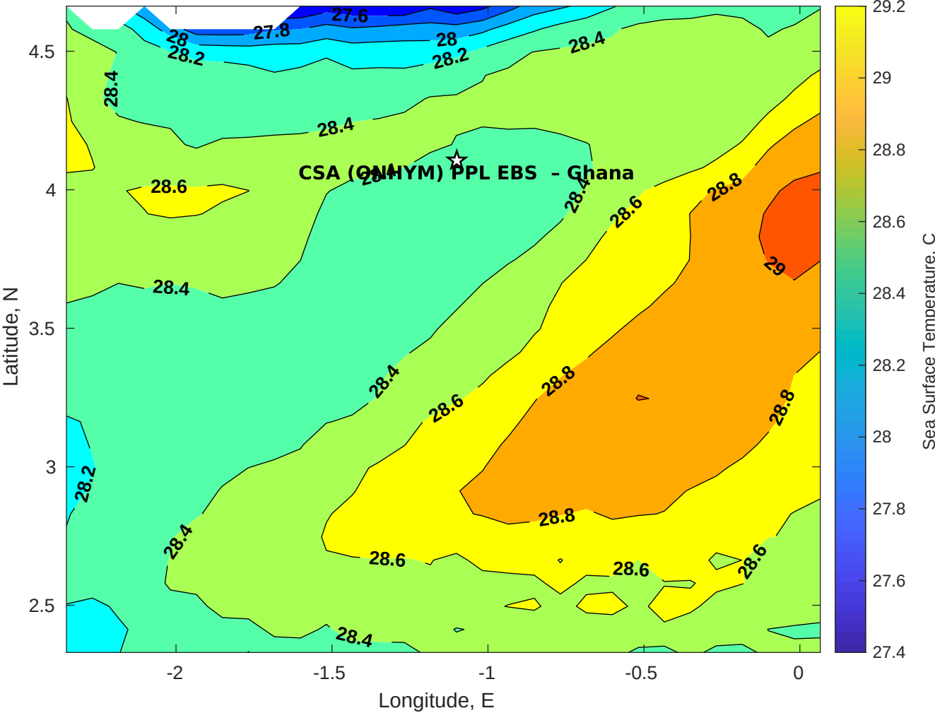
SST for CSA (ONHYM) PPL EBS - Ghana at 30-Nov-2025 00:00:00
