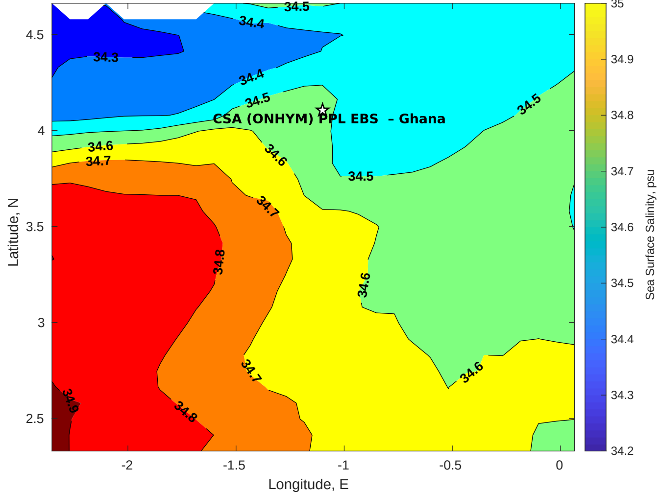
Surface Salinity for CSA (ONHYM) PPL EBS - Ghana at 30-Nov-2025 00:00:00
