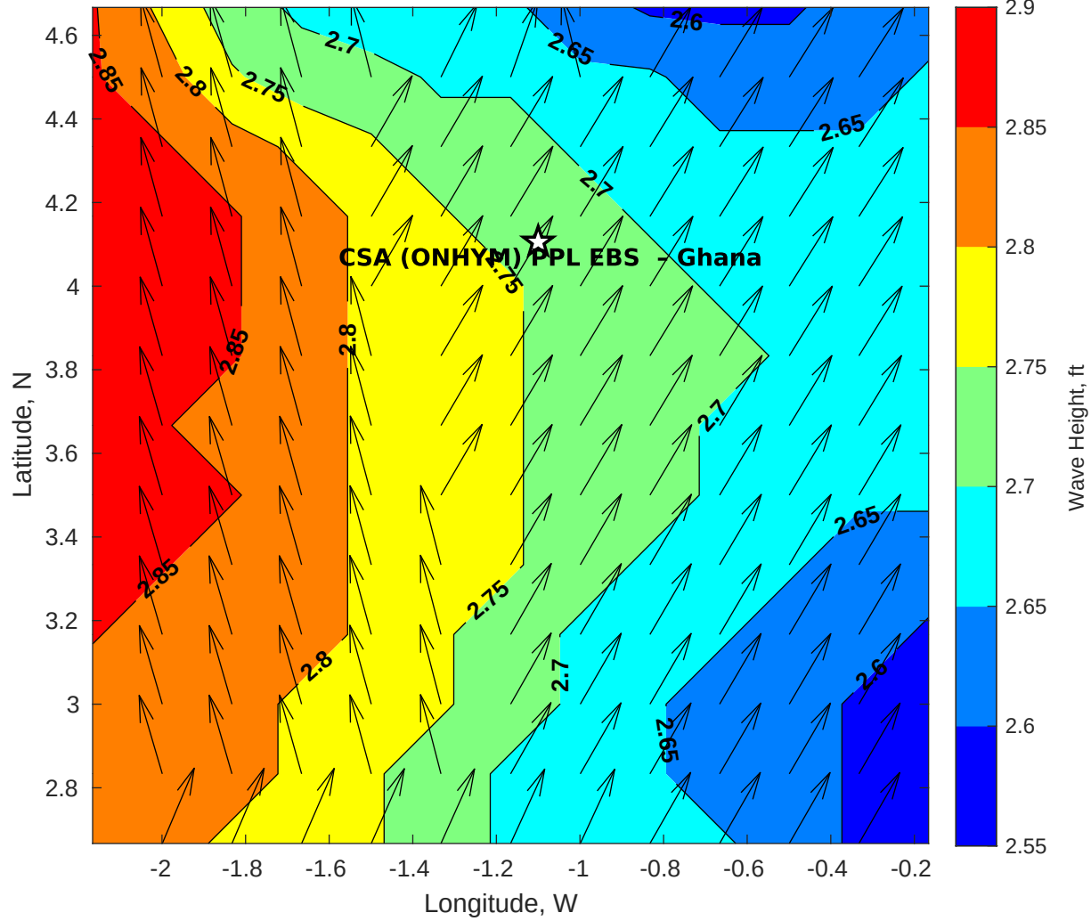
GFS Wave Height (ft) for CSA (ONHYM) PPL EBS - Ghana at 01-Dec-2025 09:00:00
