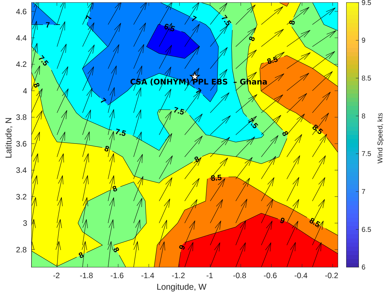
GFS Winds (kts) for CSA (ONHYM) PPL EBS - Ghana at 01-Dec-2025 09:00:00
