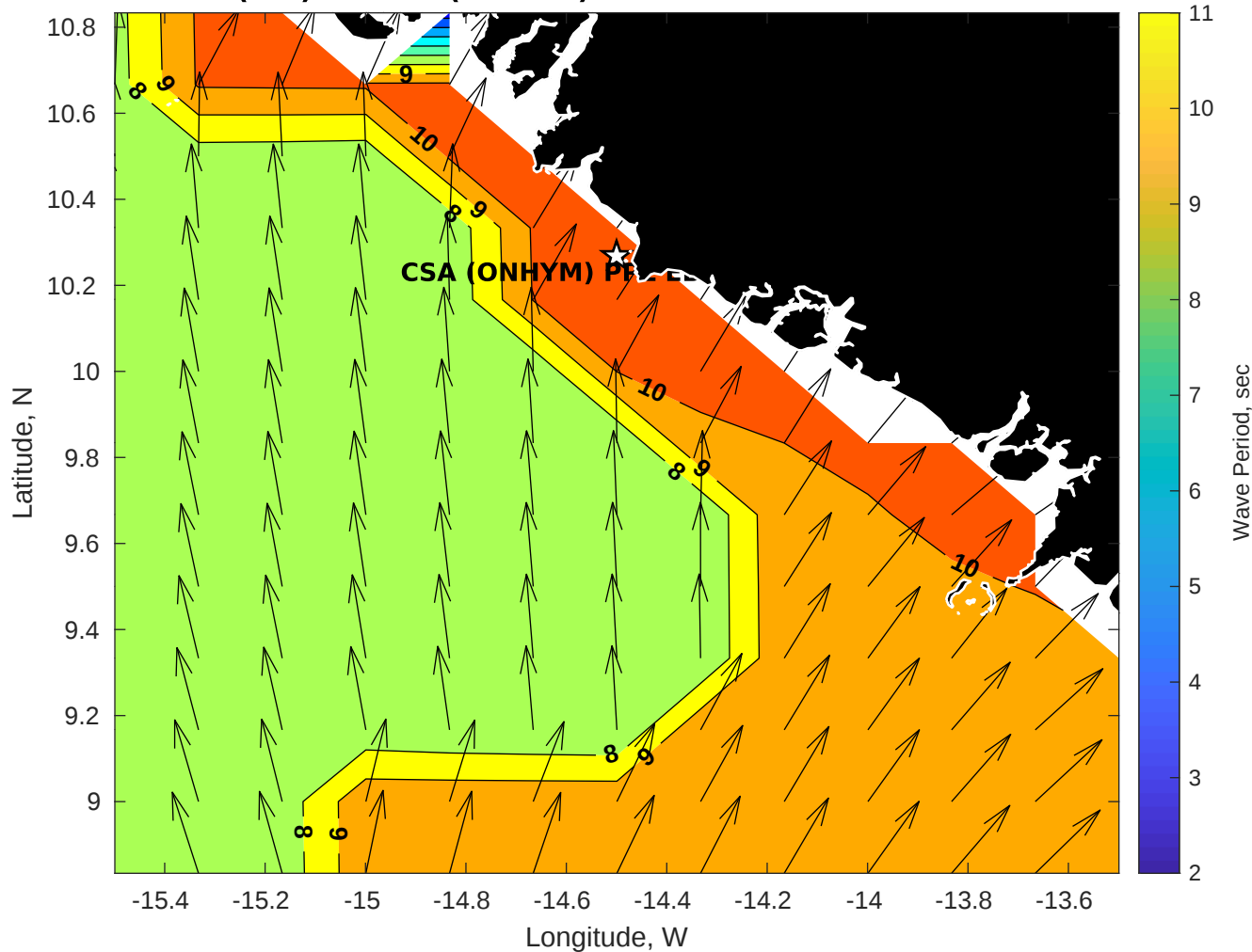
GFS Wave Period (sec) for CSA (ONHYM) PPL EBS - Guinea at 01-Dec-2025 09:00:00
