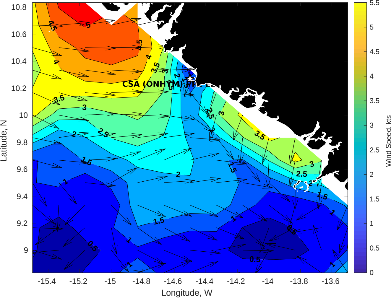
GFS Winds (kts) for CSA (ONHYM) PPL EBS - Guinea at 01-Dec-2025 09:00:00
