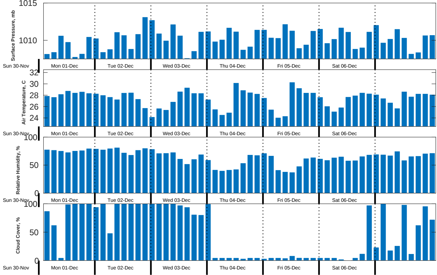
Met Forecast for CSA (ONHYM) PPL EBS - Guinea from 01-Dec-2025 00:00:00 to 08-Dec-2025 00:00:00
